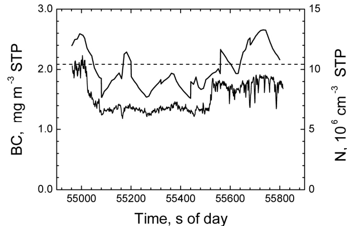
FIGURE 5 - Carbon mass concentration measured with the Multi-Angle Absorption Photometer (solid line) and with the Smoke Number method (dashed line) in an aircraft engine combustor exhaust; the lower full line indicates the number concentration of combustion particles (Reference 33)
