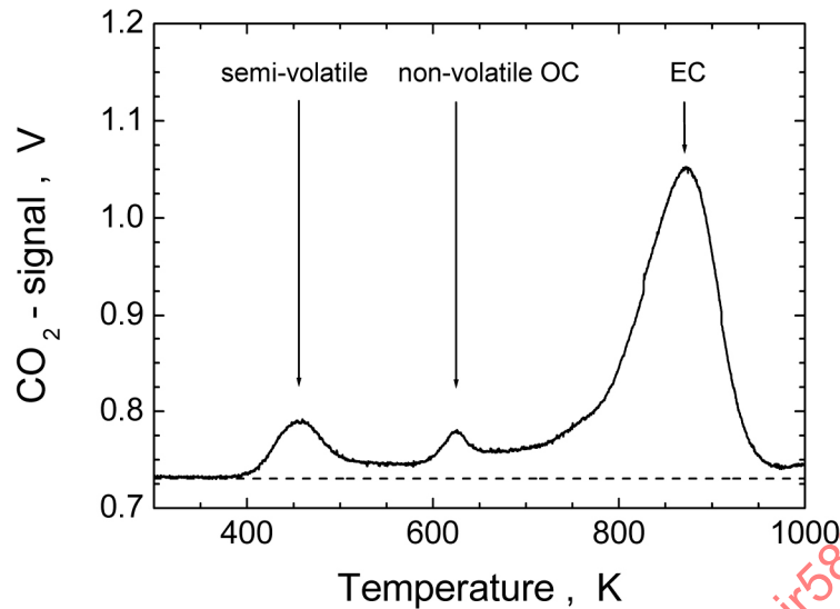
FIGURE 1 - Evolving CO 2 as a function of the sample heating temperature for a combustor particulate matter sample; semi-volatile OC oxidizes at 450 K, nonvolatile OC at 600 K, and elemental carbon above 700 K (Reference 34)
