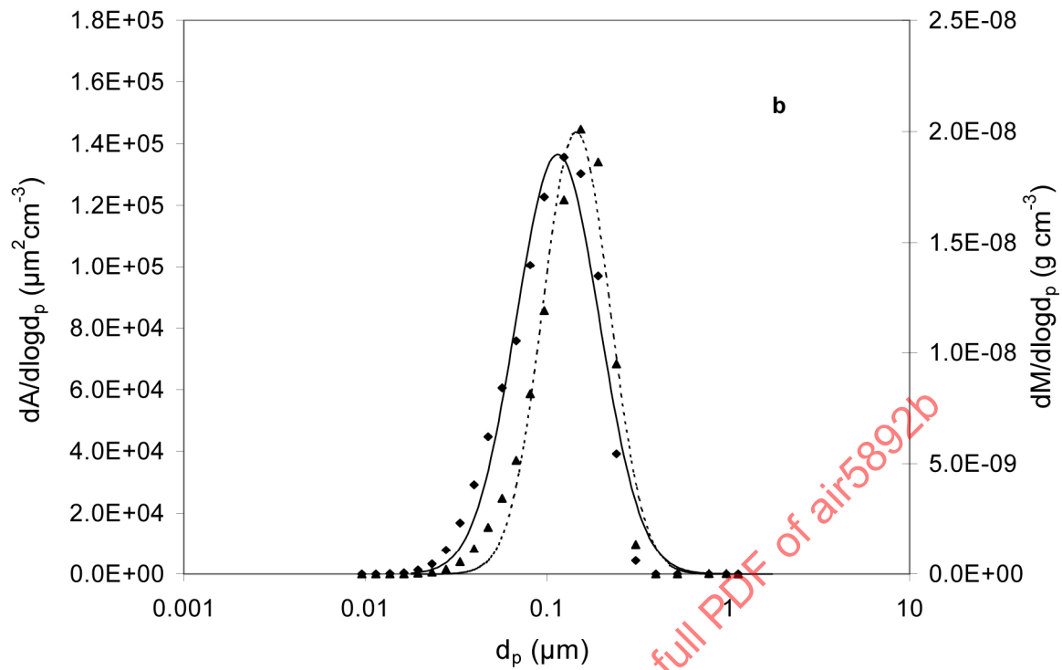
FIGURE 12 - Computed Surface Area and Mass for Turbine Engine Particle Emissions
