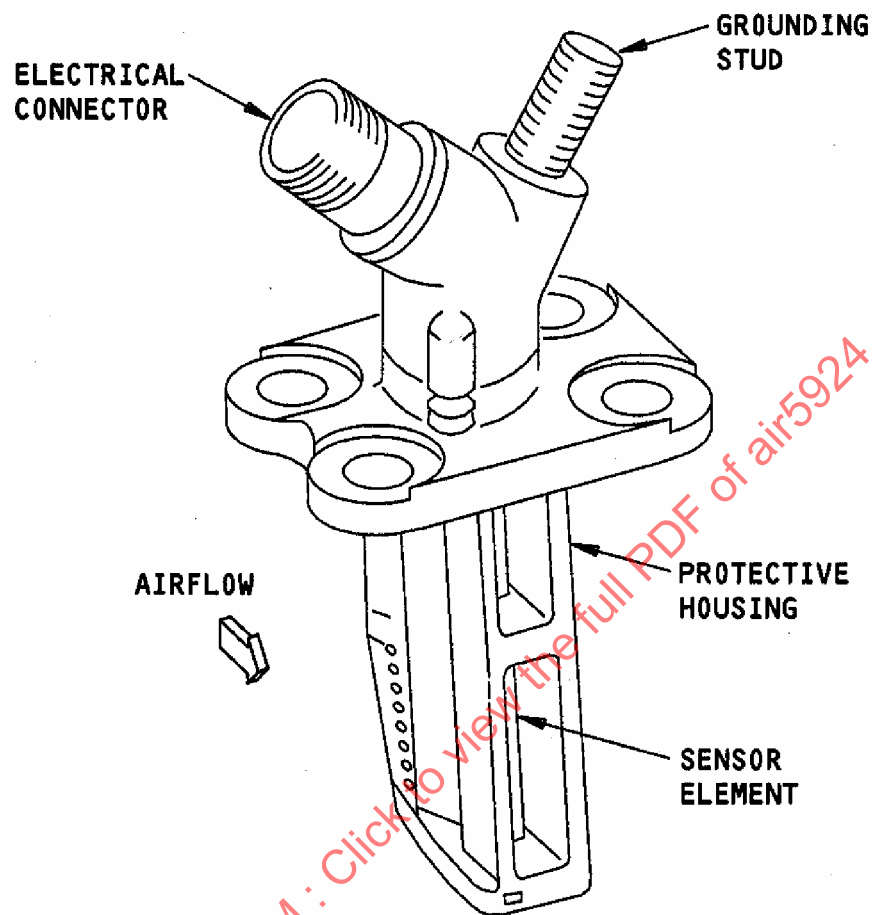
FIGURE 17 - Non-Aspirated TAT Probe (Courtesy of Rosemount Aerospace Inc. The external shape of the TAT probe in the figure is a registered trademark of Rosemount Aerospace Inc.)
