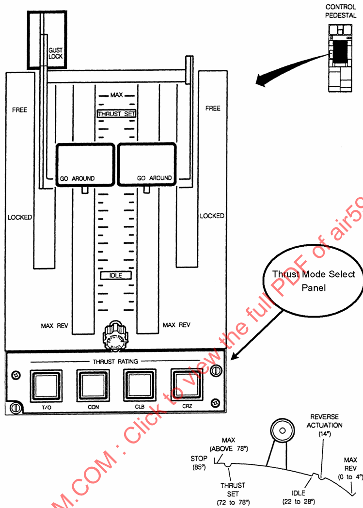
FIGURE 10 - Thrust Rating Selection Panel
