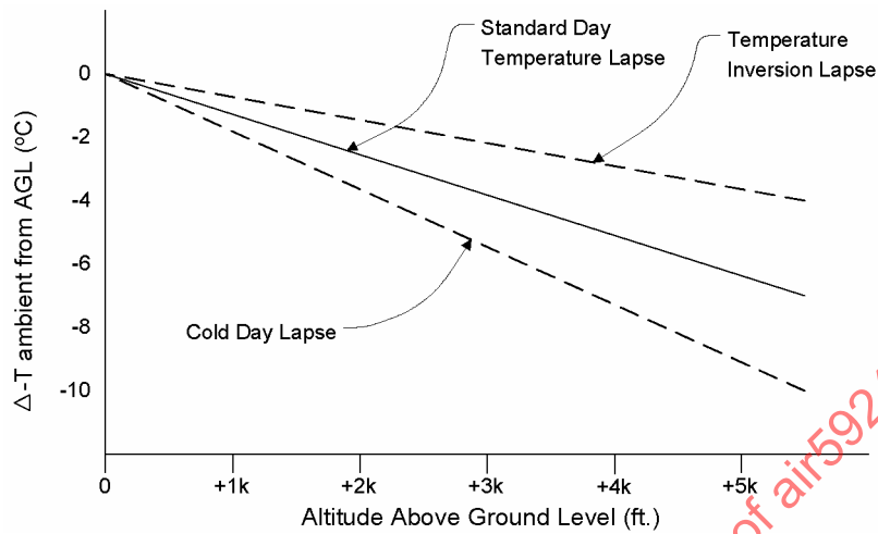
FIGURE 11a - Ambient Temperature Lapse from AGL
