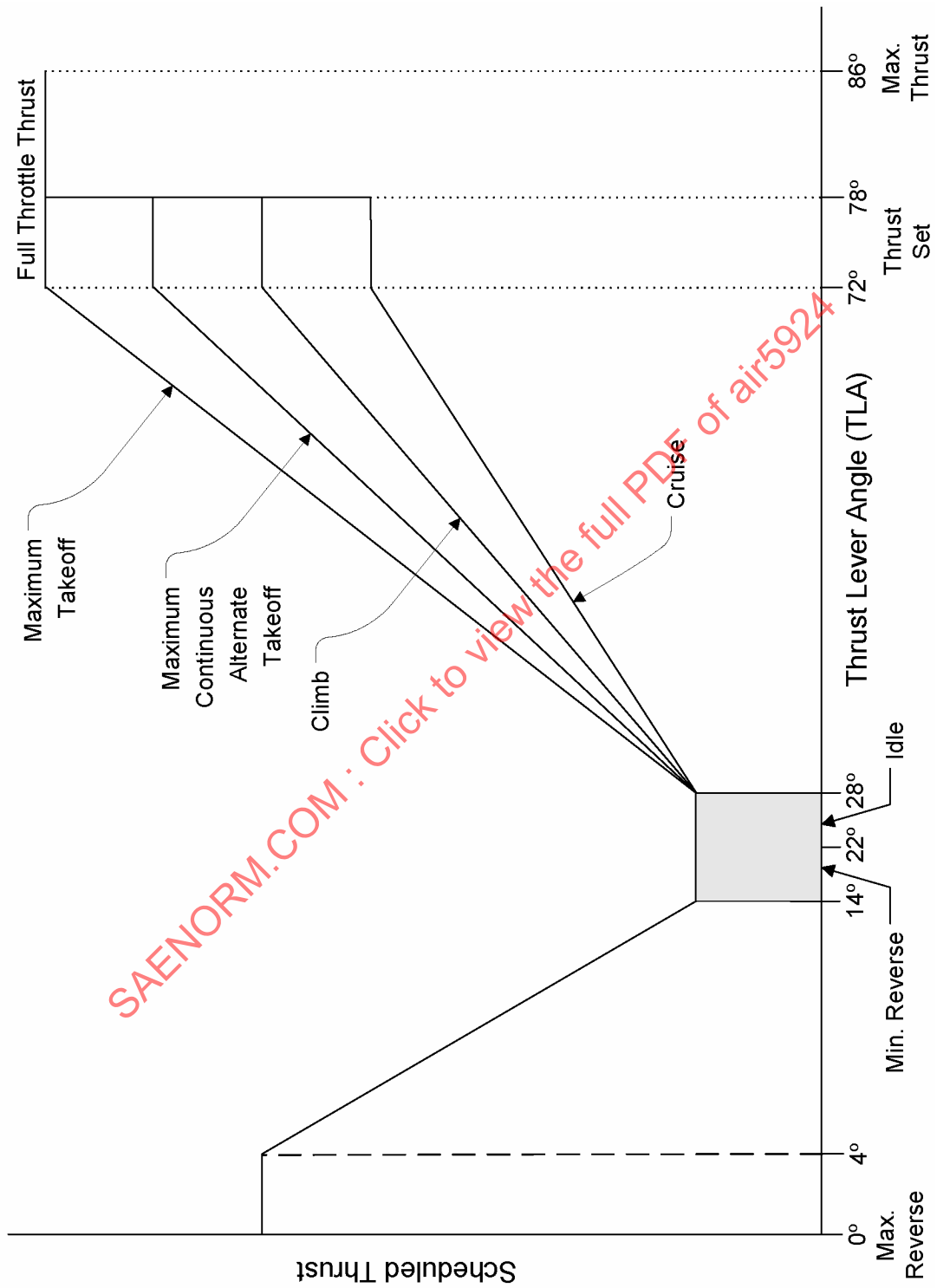
FIGURE 9 - Thrust Schedule Using Mode Selection Panel
