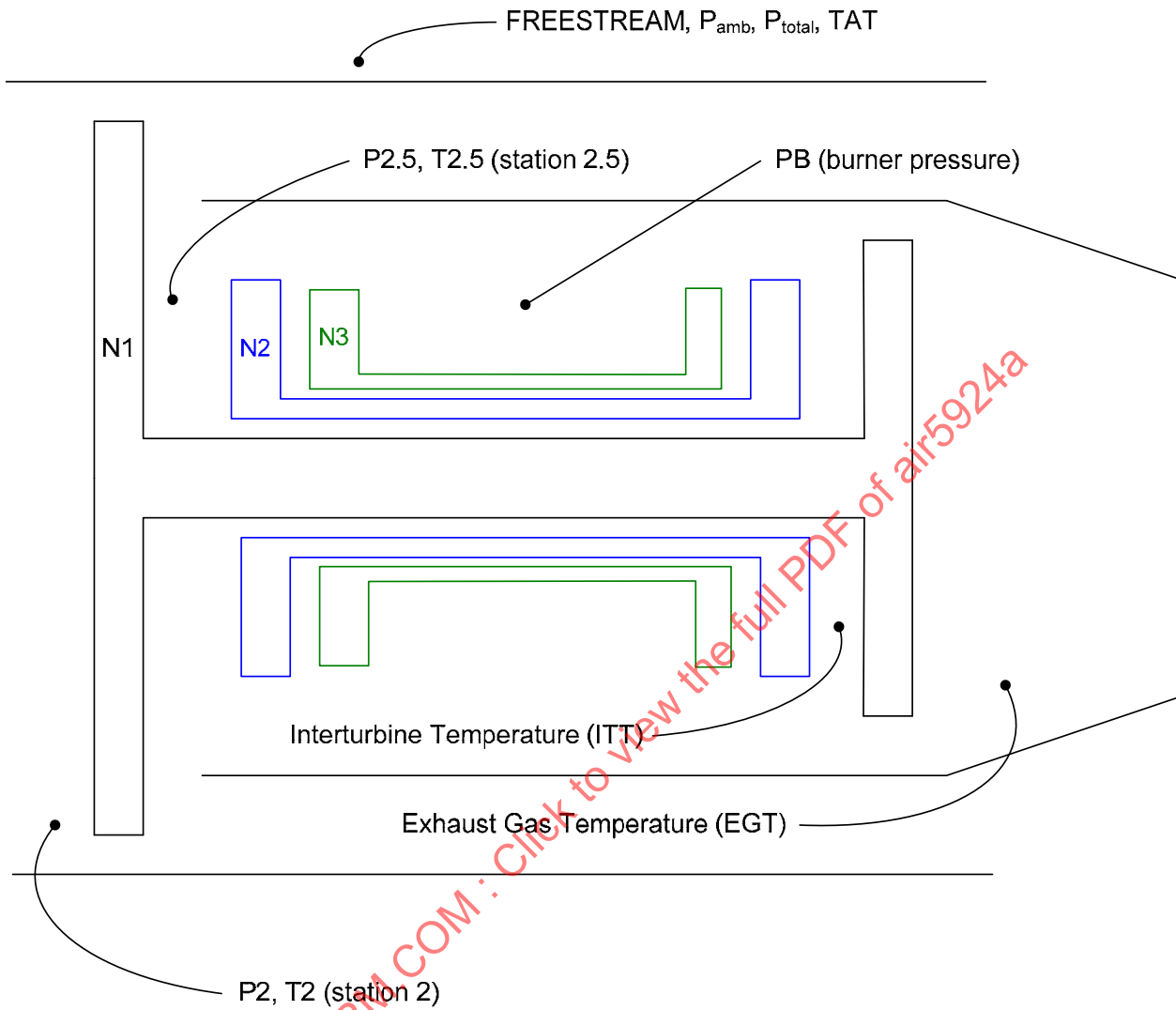
FIGURE 1 - STATION DEFINITIONS USED HEREIN
