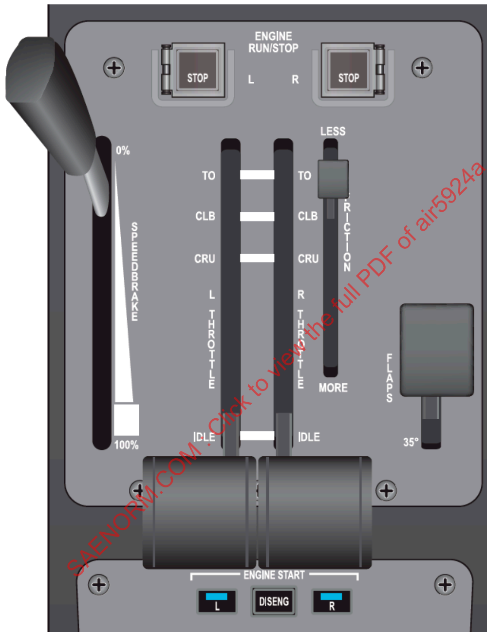
FIGURE 9 - A DETENTED OR "FIXED POSITION" THROTTLE QUADRANT
