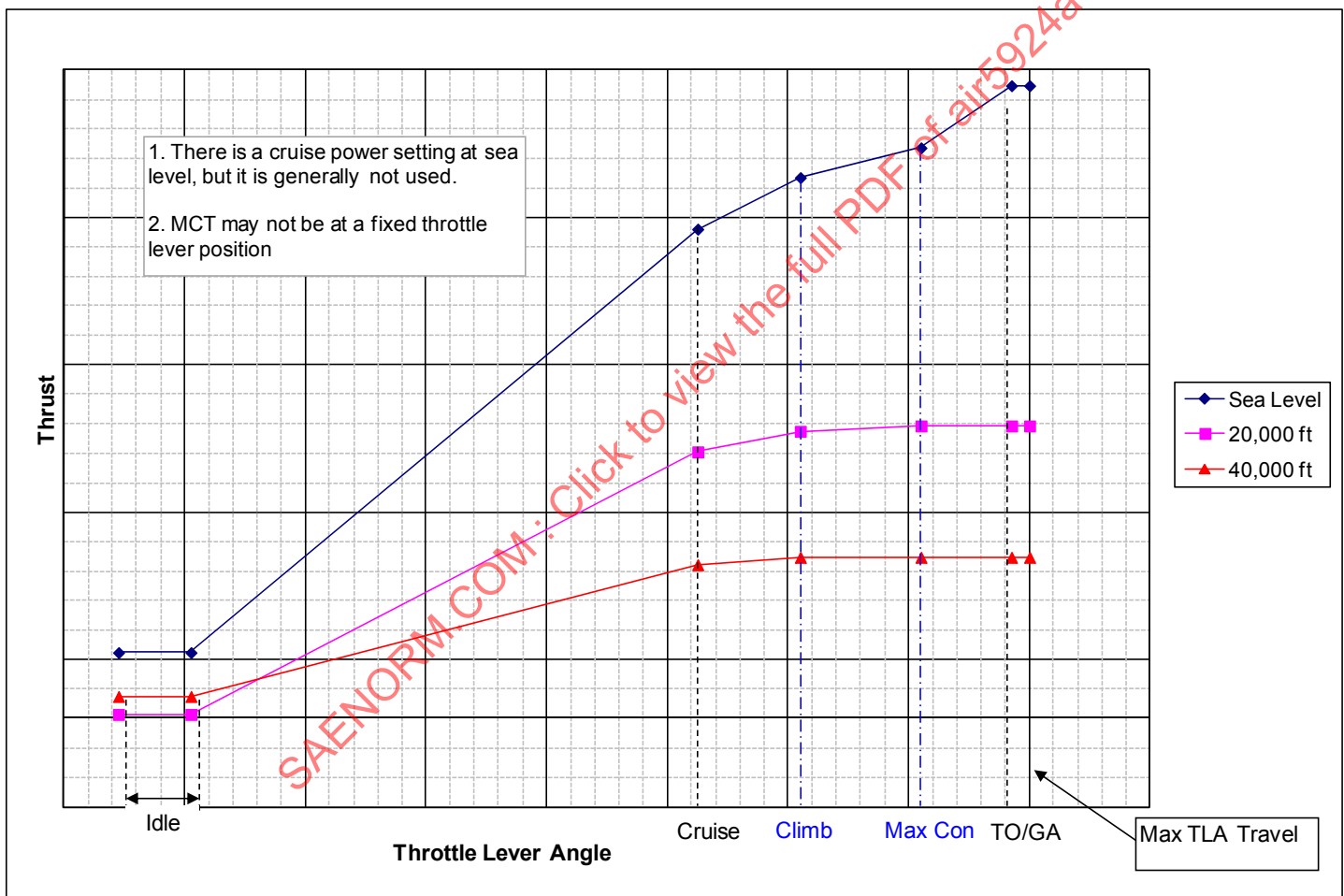
FIGURE 11 - THRUST VERSUS THROTTLE LEVER ANGLE WITHOUT DETENTS
