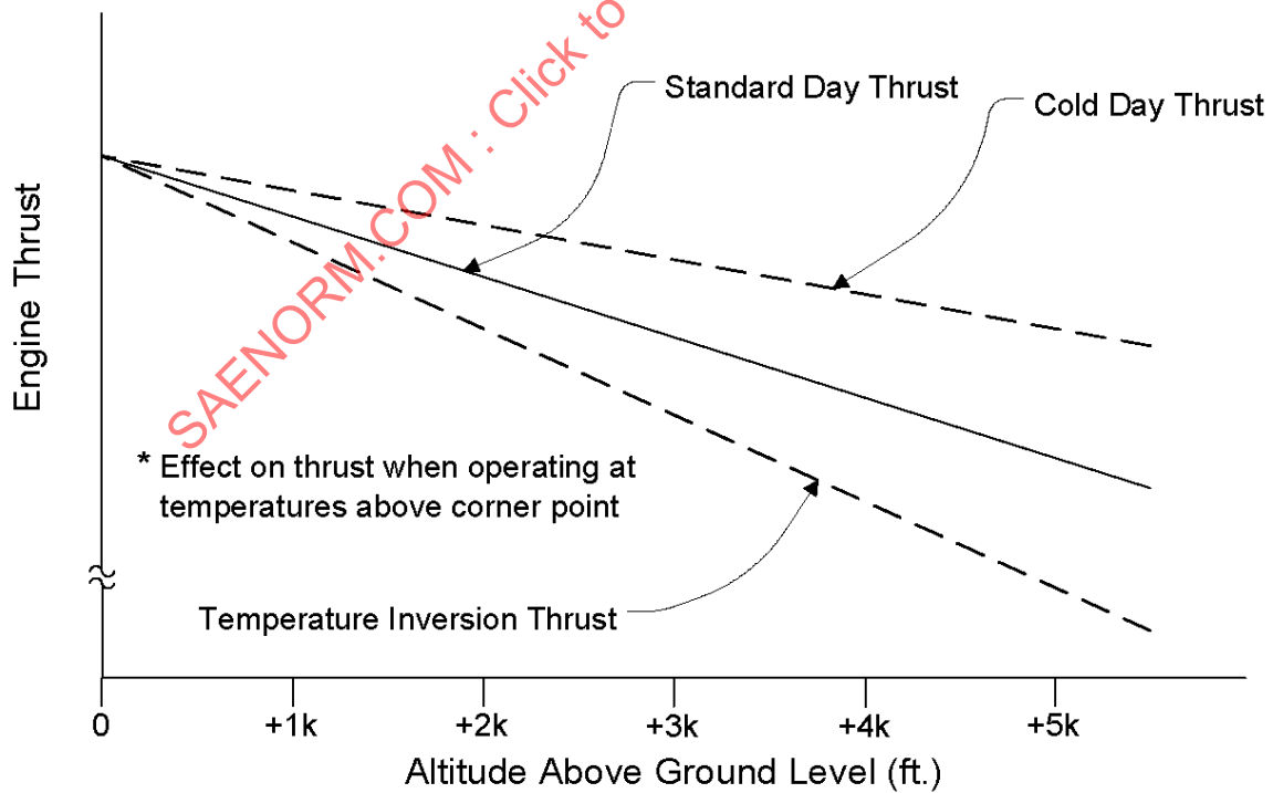
FIGURE 16 - THRUST AS A FUNCTION OF AMBIENT TEMPERATURE AND ALTITUDE INCREASE AT CONSTANT MACH NUMBER
