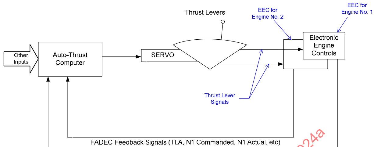
FIGURE 18 - MOVING THRUST LEVER AUTO-THRUST SYSTEM
