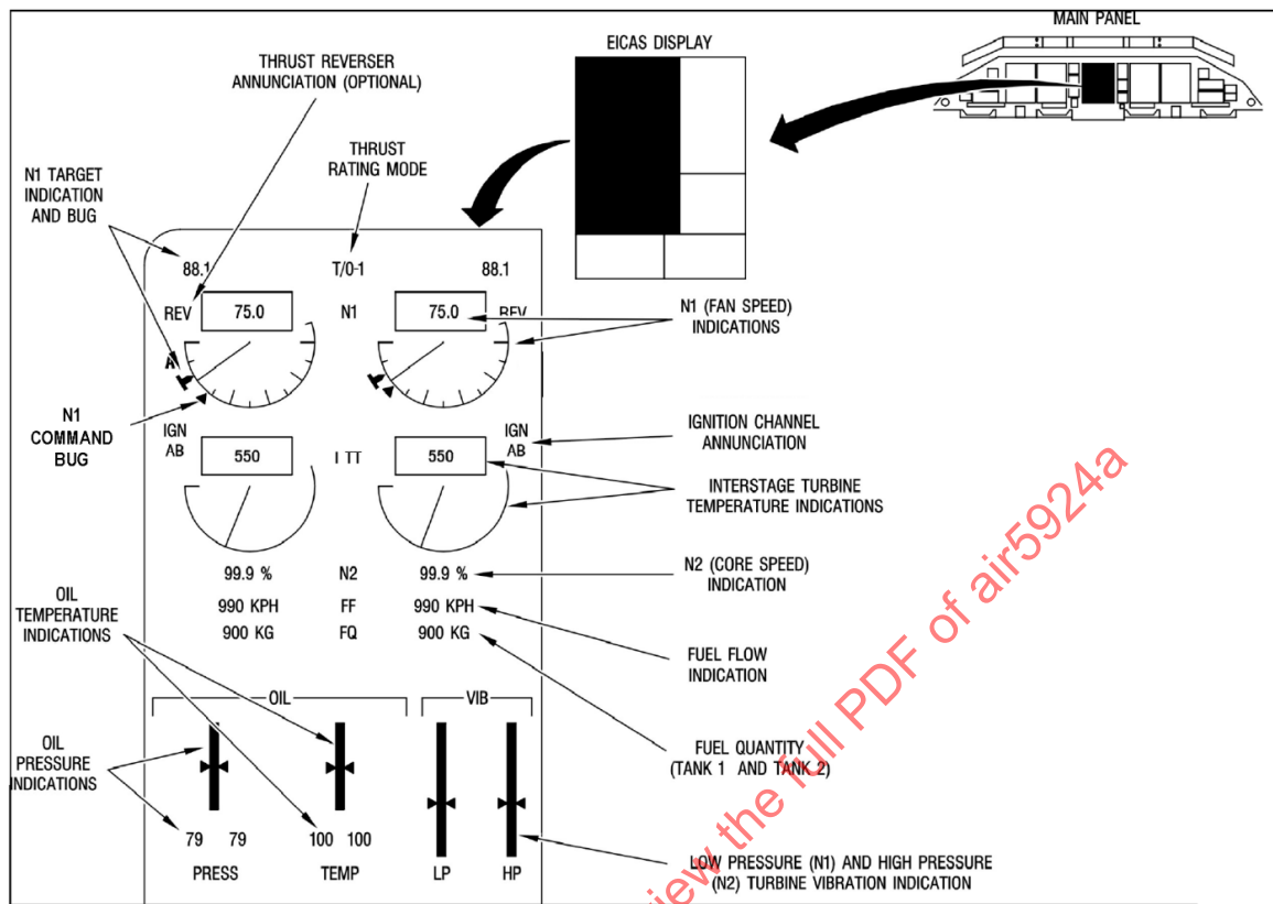
FIGURE 27 - TYPICAL PRESENTATION OF POWERPLANT DATA
