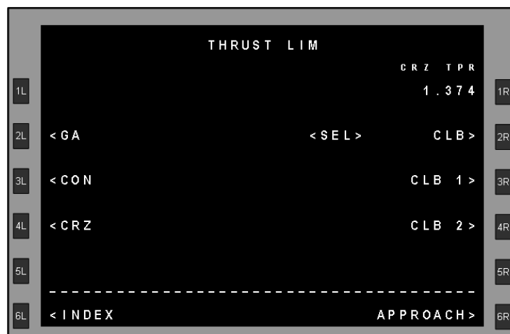
FIGURE 14 - TYPICAL THRUST RATING SELECTION DISPLAY IN-FLIGHT
