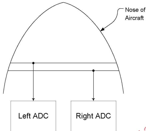
FIGURE 22 - TYPICAL CROSS-MANIFOLDED BODY STATIC PRESSURE SENSING CONFIGURATION
