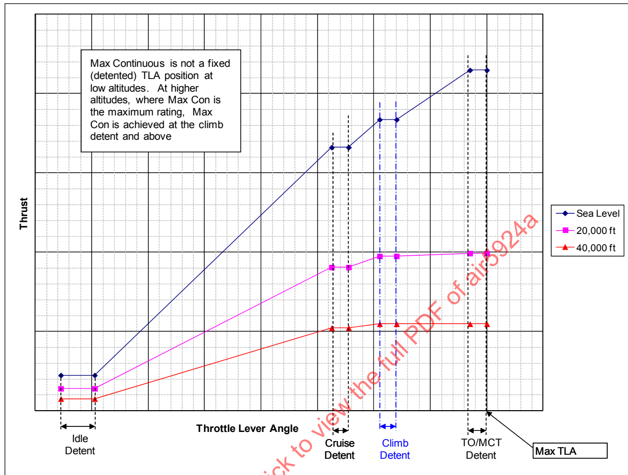
FIGURE 7 - TYPICAL ALTITUDE DEPENDENT THRUST SCHEDULES VERSUS THRUST LEVER POSITION
