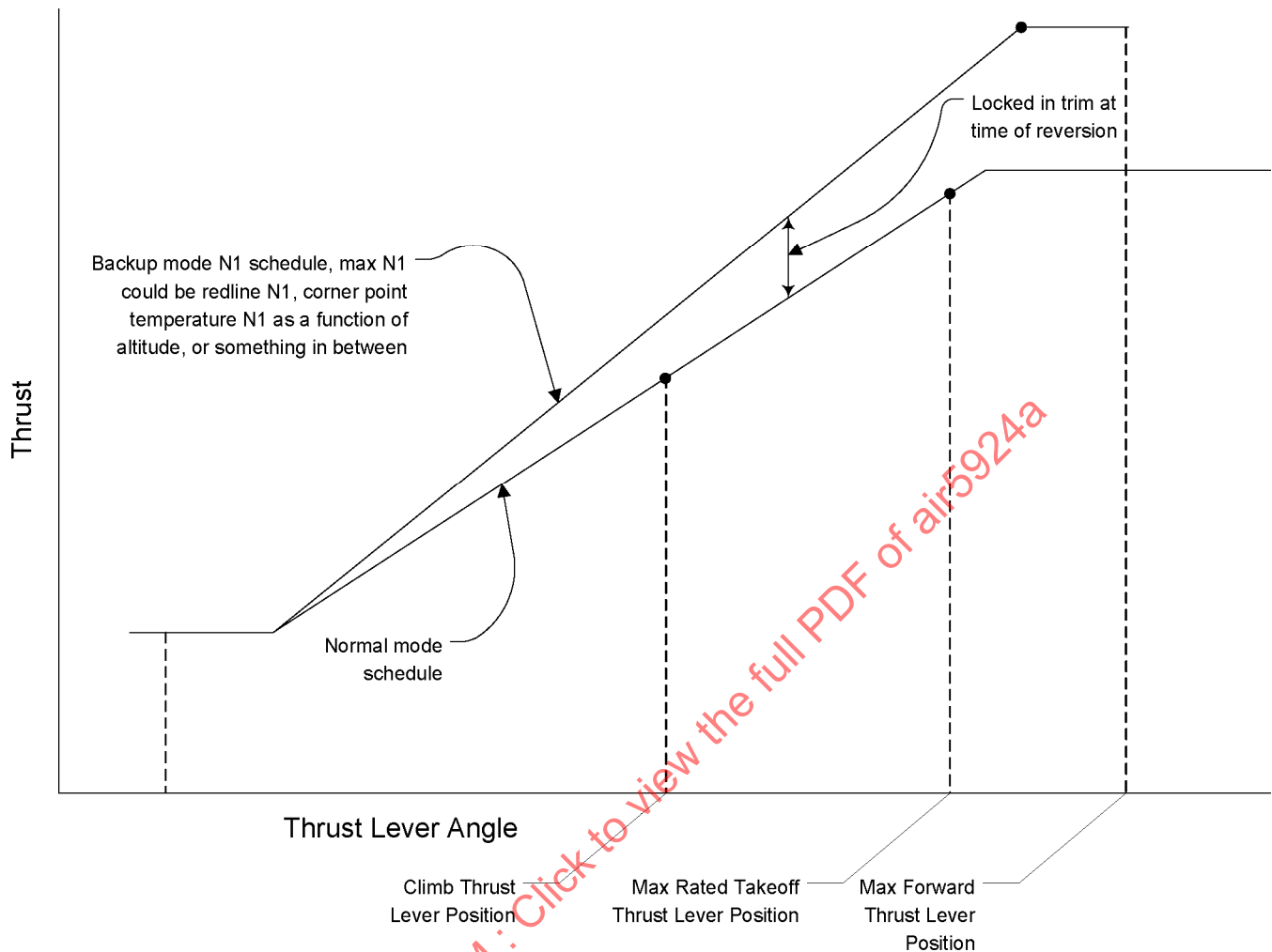
FIGURE 4 - NORMAL MODE THRUST SCHEDULE AS COMPARED WITH TYPICAL ALTERNATE (OR BACKUP) MODE SCHEDULE FOR FORWARD THRUST
