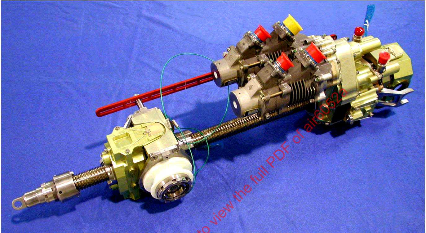
Figure 9 - Bombardier Challenger 300 series trimmable horizontal stabilizer actuator
