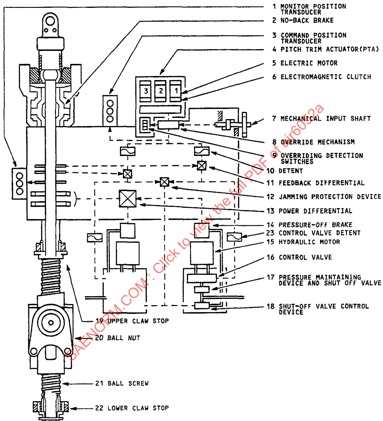
Figure 3 - Airbus A330-200/-300/A340-200/-300 trimmable horizontal stabilizer actuator schematic diagram
