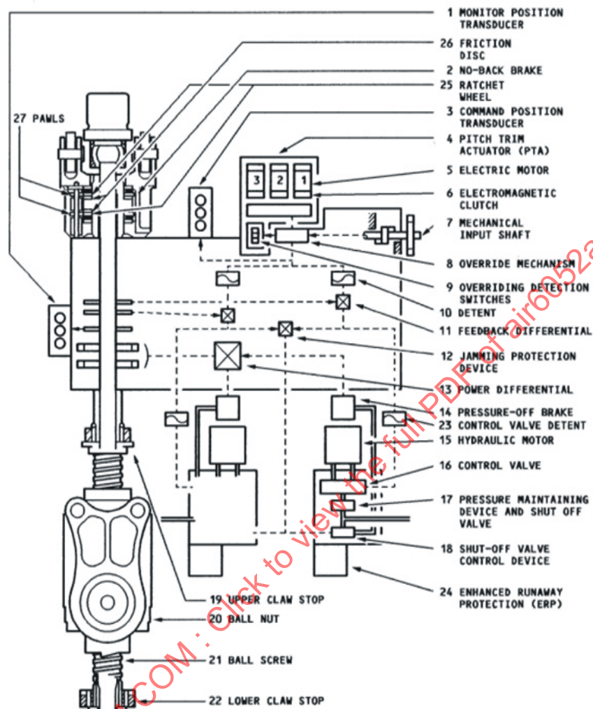
Figure 4 - Airbus A340-500/-600 trimmable horizontal stabilizer actuator schematic diagram
