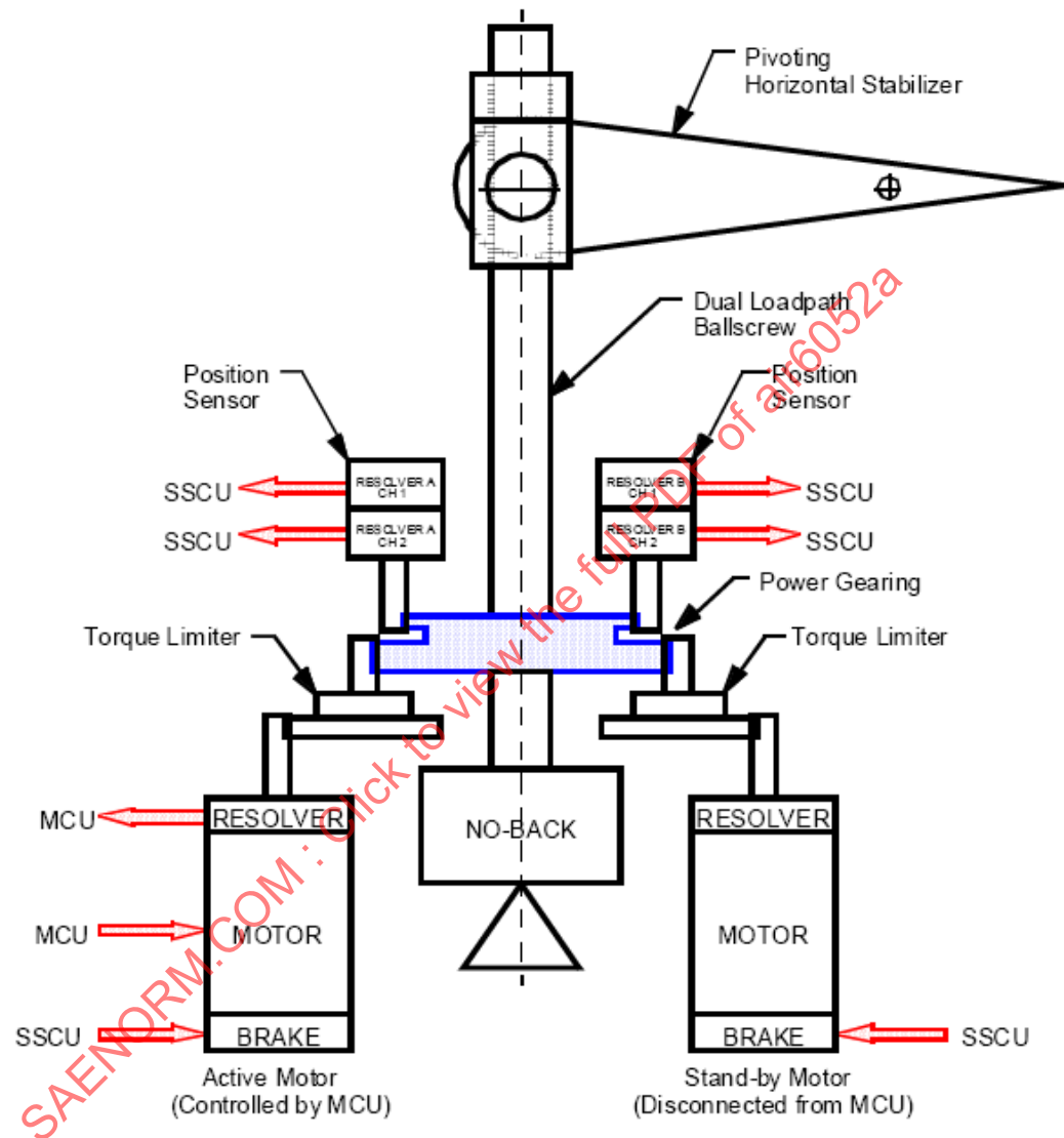
Figure 10 - Bombardier CRJ-700/-900/-1000 trimmable horizontal stabilizer actuator schematic diagram
