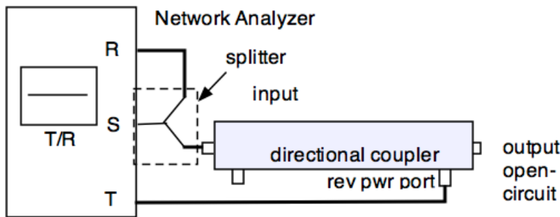
Figure 5 - Directional coupler reverse power coupling factor measurement
