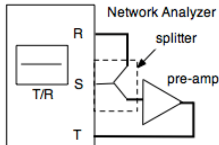
Figure 10 - Low noise preamplifier gain measurement
