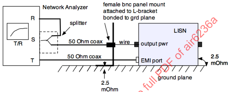
Figure 2 - LISN insertion loss measurement set-up
