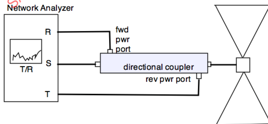
Figure 12 - Antenna vswr measurement
