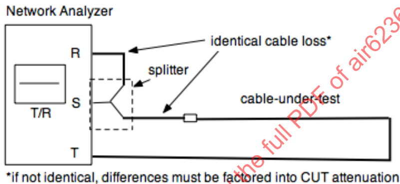
Figure 9 - Cable loss measurement
