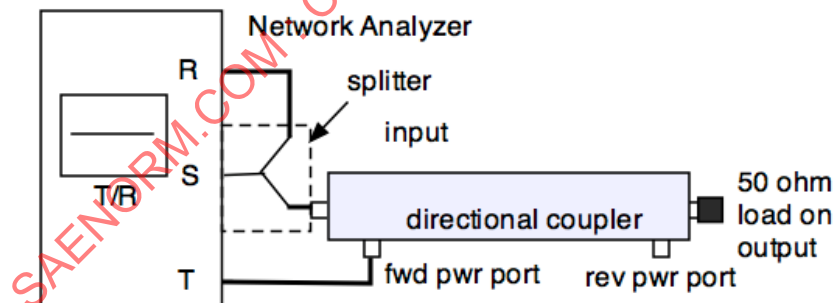
Figure 4 - Directional coupler forward power coupling factor measurement
