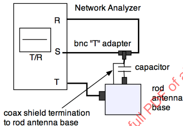
Figure 11 - 41 inch rod antenna base transducer factor measurement
