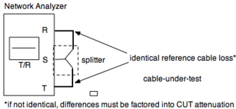
Figure 8 - Reference cable loss measurement
