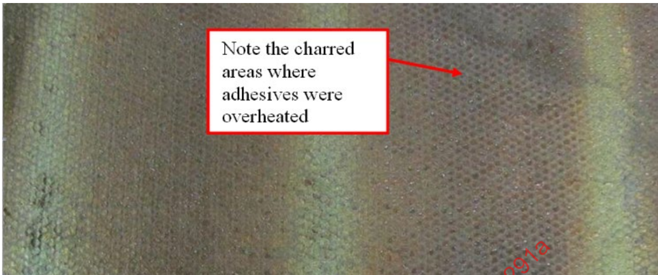
Figure 31 - Example of a thermocouple failure during repair cure
