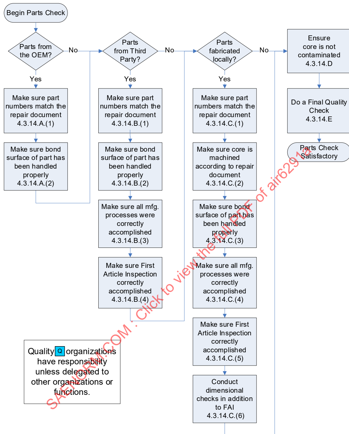
Figure 15 - Parts check process flow
