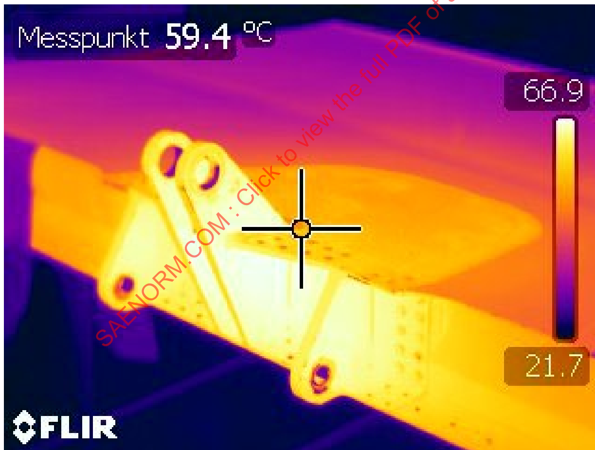
Figure 4 - Thermal image demonstrates how a metallic fitting acts as a heat sink
