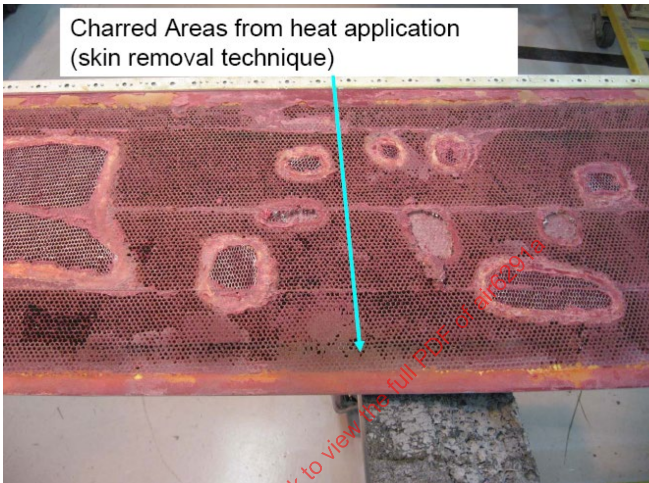
Figure 6 - Example of overheating during skin removal
