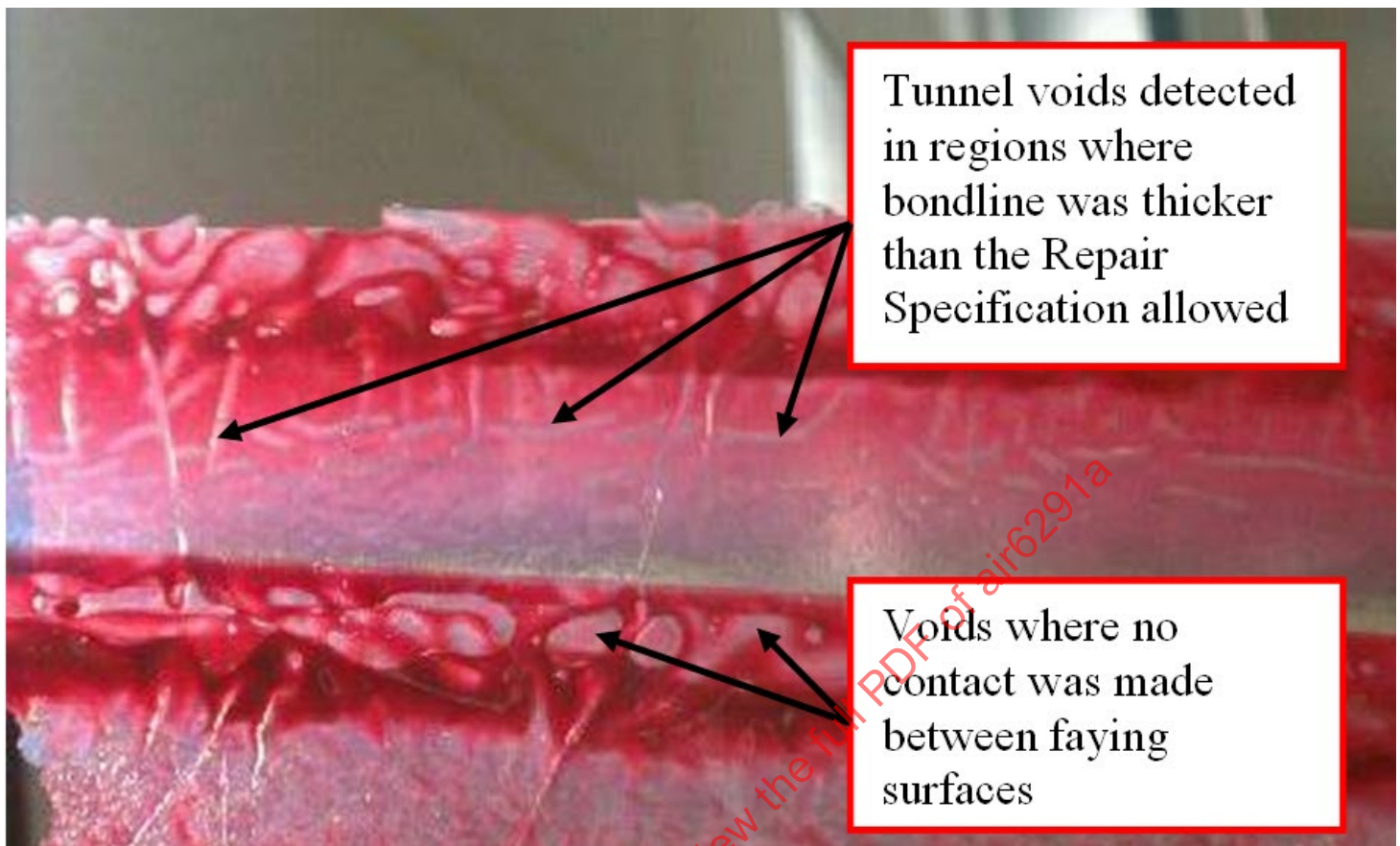
Figure 25 - Tunnel voids shown at the interface between a tool side skin and spar flange for a wedge assembly
