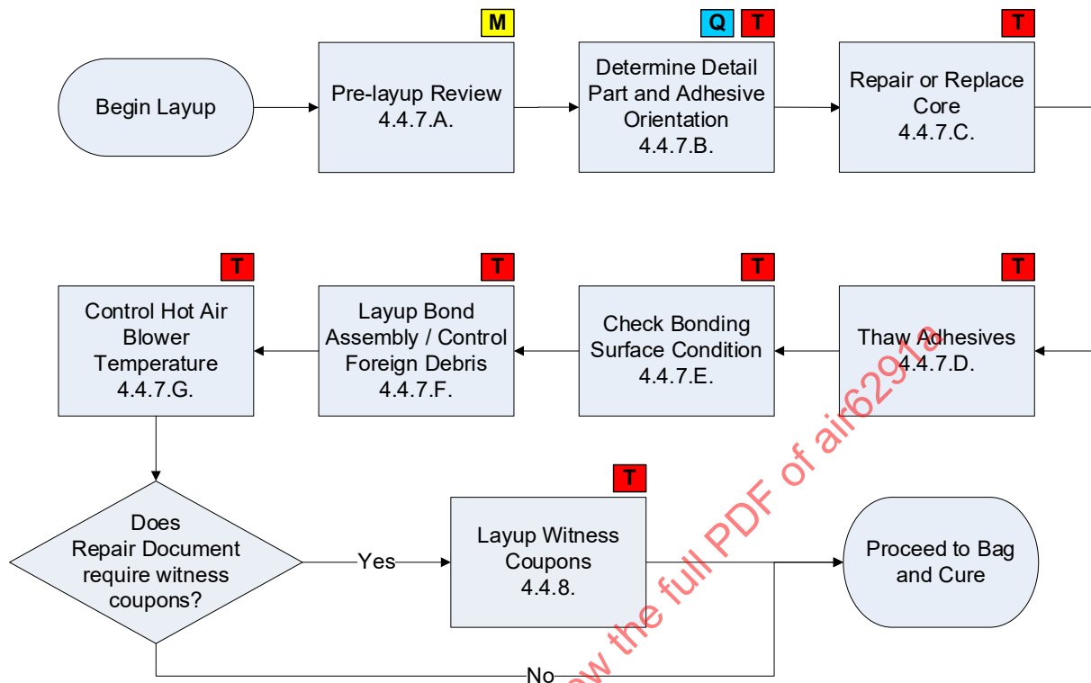
Figure 28 - Layup process flow
