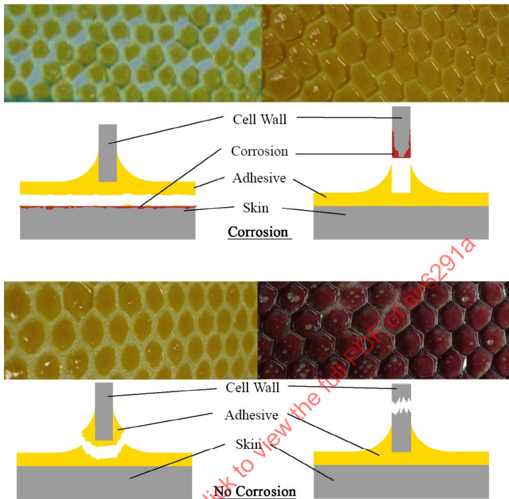
Figure 9 - Examining peeled skin and residual core for evidence of corrosion
