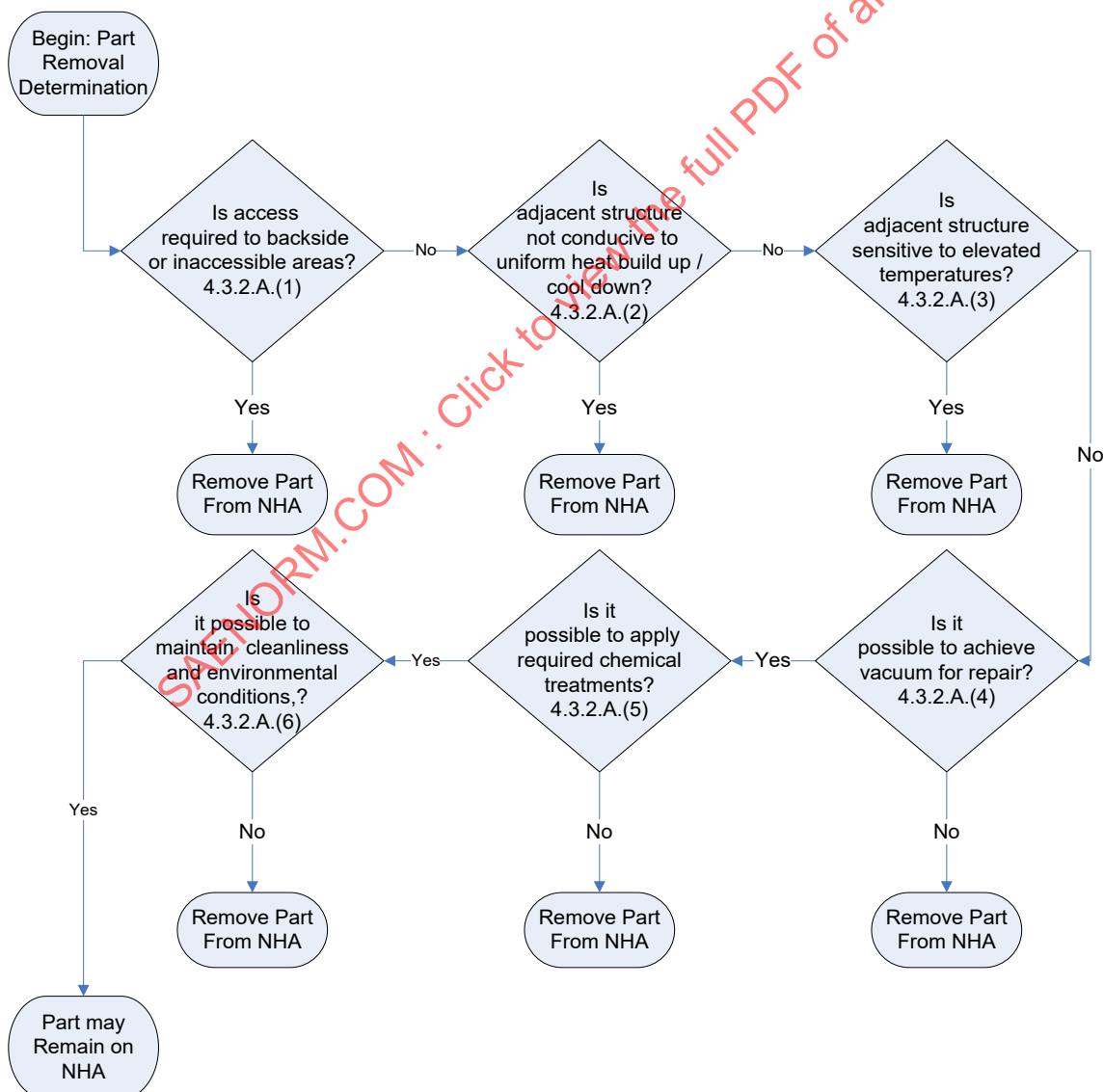
Figure 3 - Part removal decision flow
