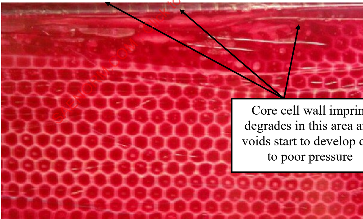
Figure 23 - Example of nonuniform core imprint
