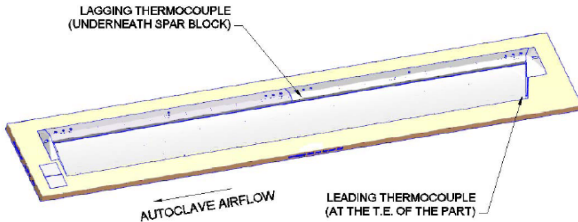
Figure 17 - Thermocouple diagram showing placement of thermocouples on tool
