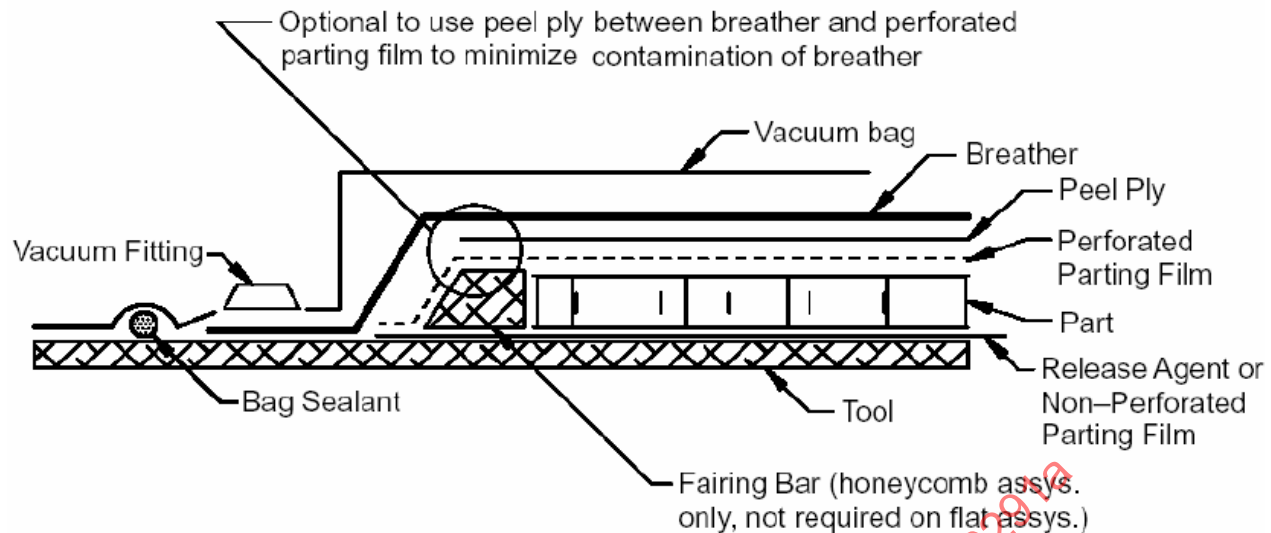
Figure 30 - Typical bagging schedule for aluminum bonded repairs
