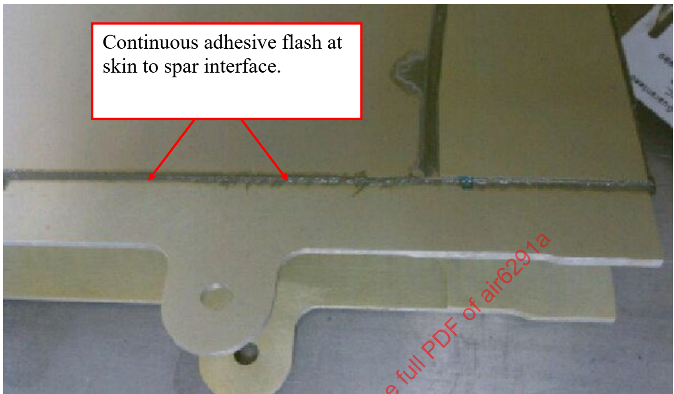
Figure 33 - Example of continuous adhesive flash along a bond line edge
