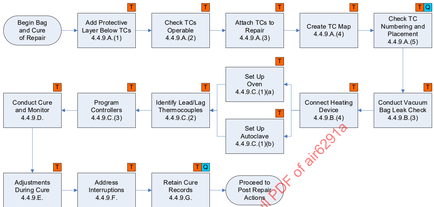
Figure 29 - Bag and cure process flow
