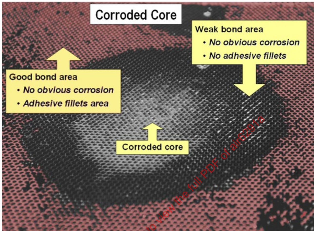
Figure 7 - Corrosion of aluminum honeycomb core resulting in a weak bond area
