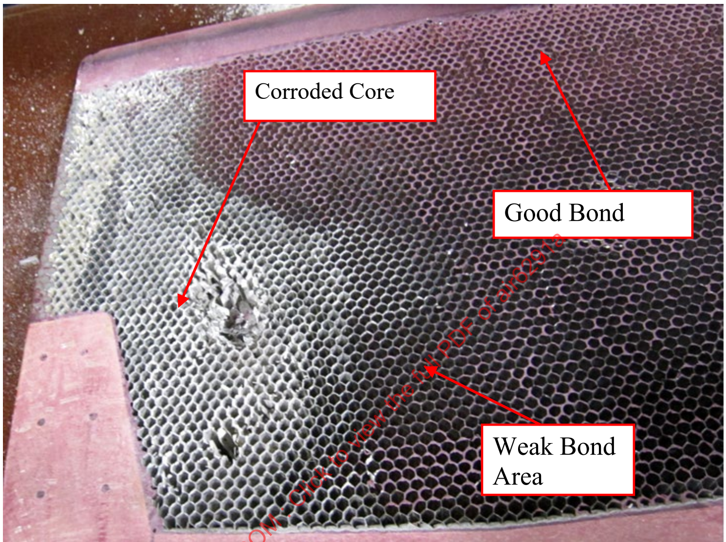
Figure 8 - Example of corroded core weak bond/good bond areas. Note that the corrosion area corresponds with a typical moisture ingress path (exposed honeycomb core edge with only a sealant close-out).
