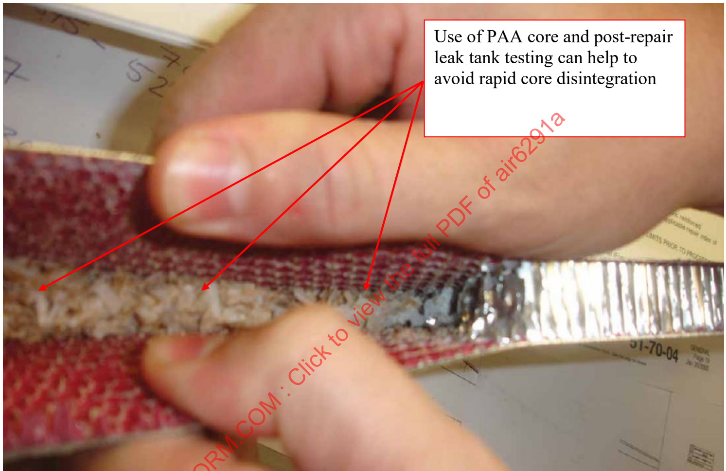
Figure 14 - Non-PAA aluminum honeycomb core found disintegrated after less than 2 years flight time
