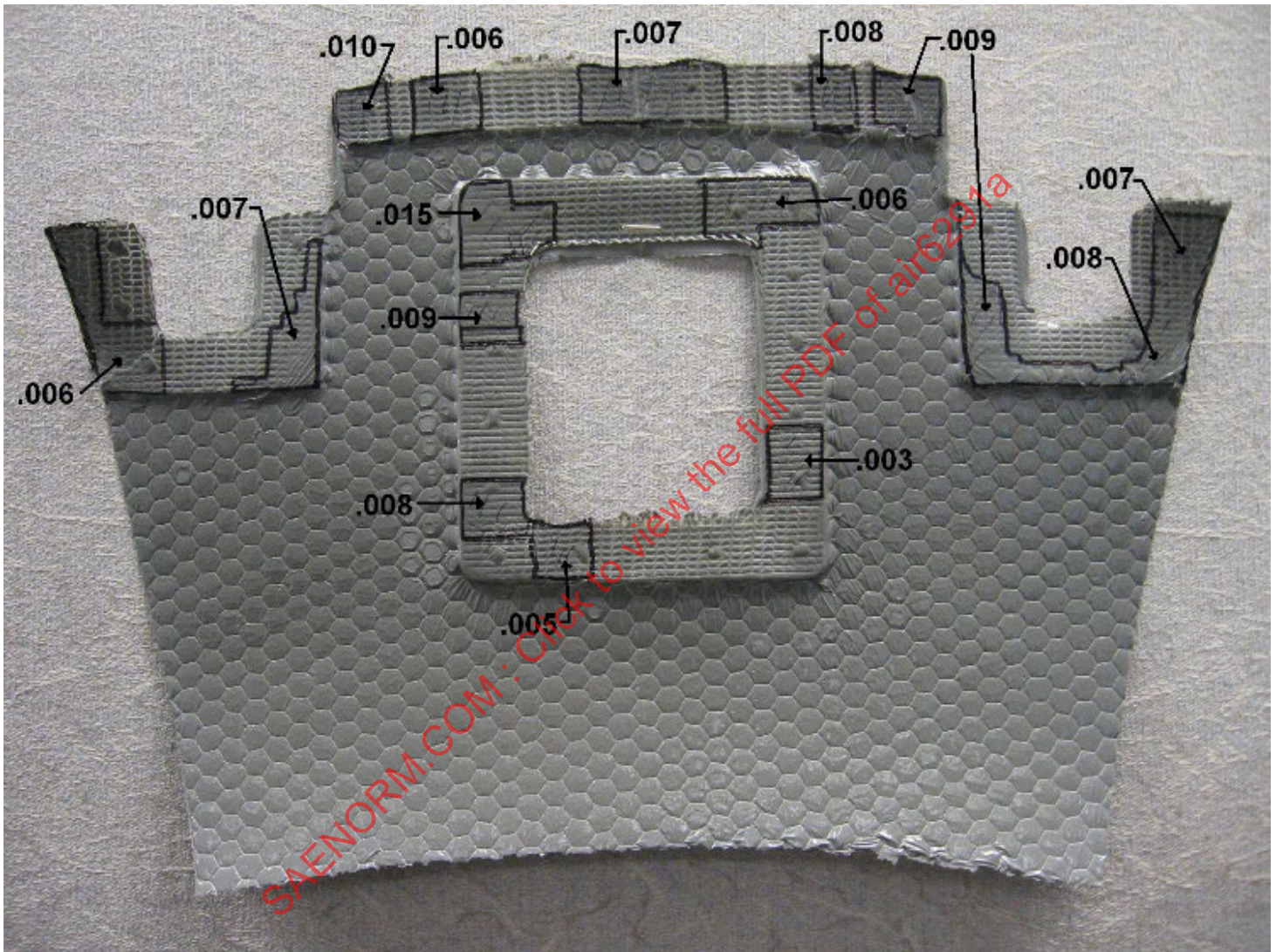
Figure 24 - Example of a verification film test cured out and circled thickness indications in areas that appear dark when exposed to a light source
