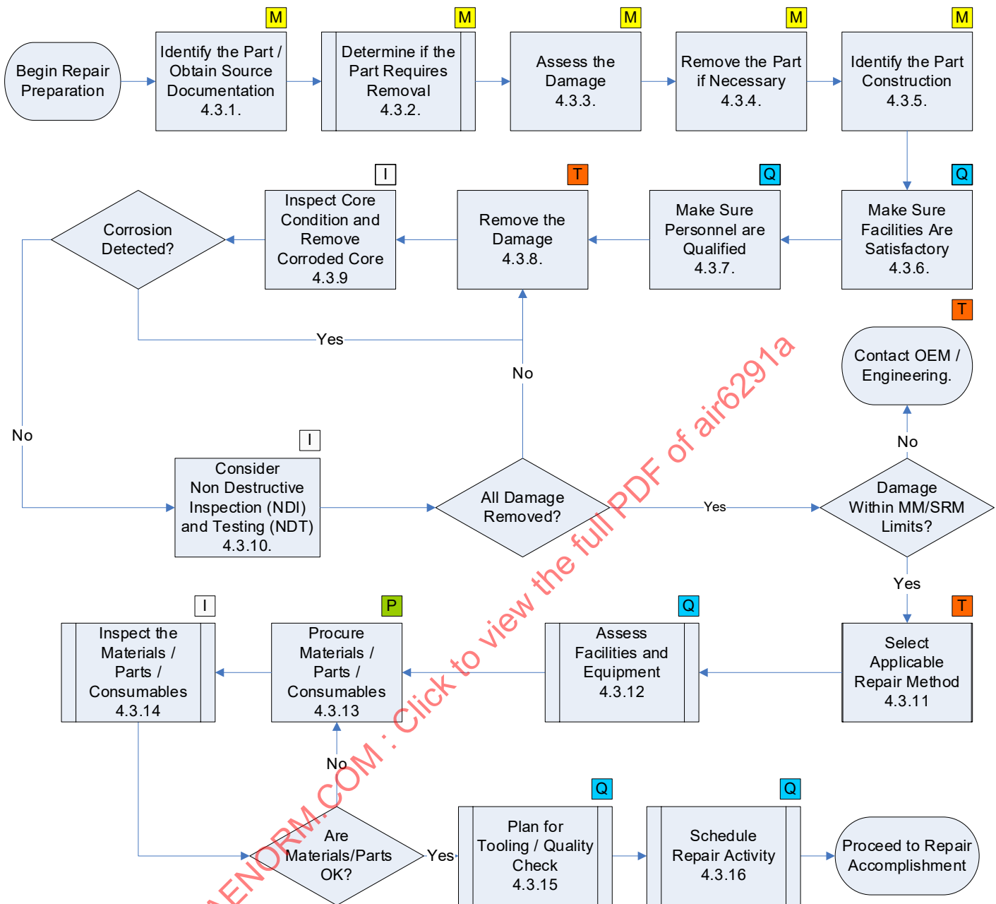
Figure 2 - Repair preparation decision flow
