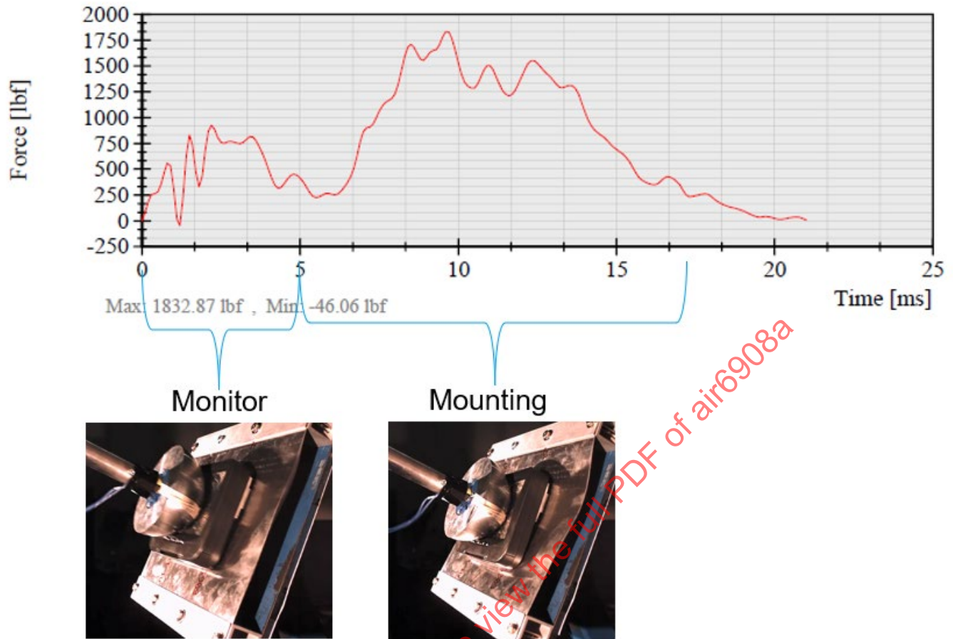
Figure 21 - Frangibility testing - general characteristics
