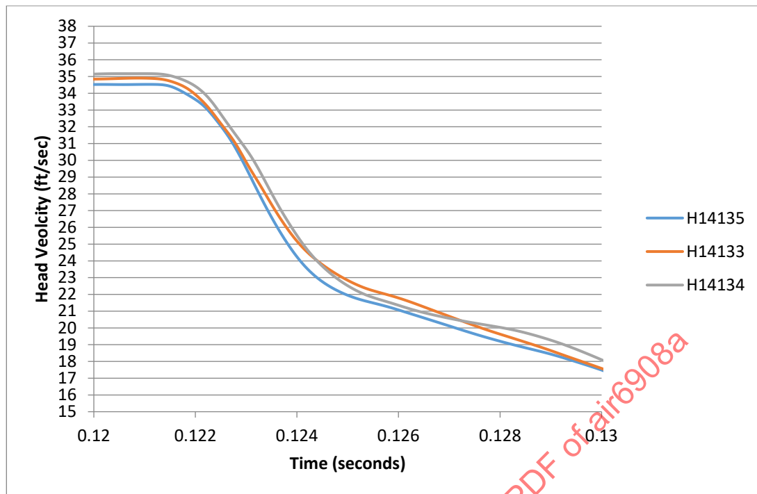
Figure C8 - Configuration #3 ATD head velocity
