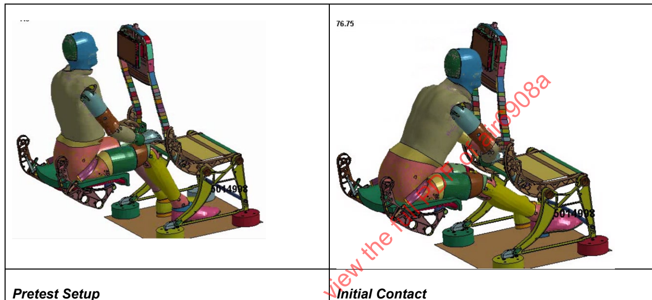
Figure G1 - Collins Aerospace row-to-row HIC simulation screenshots
