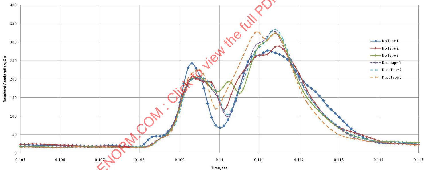
Figure I2 - Head acceleration over time, baseline versus duct tape monitor configuration, impact location #1
