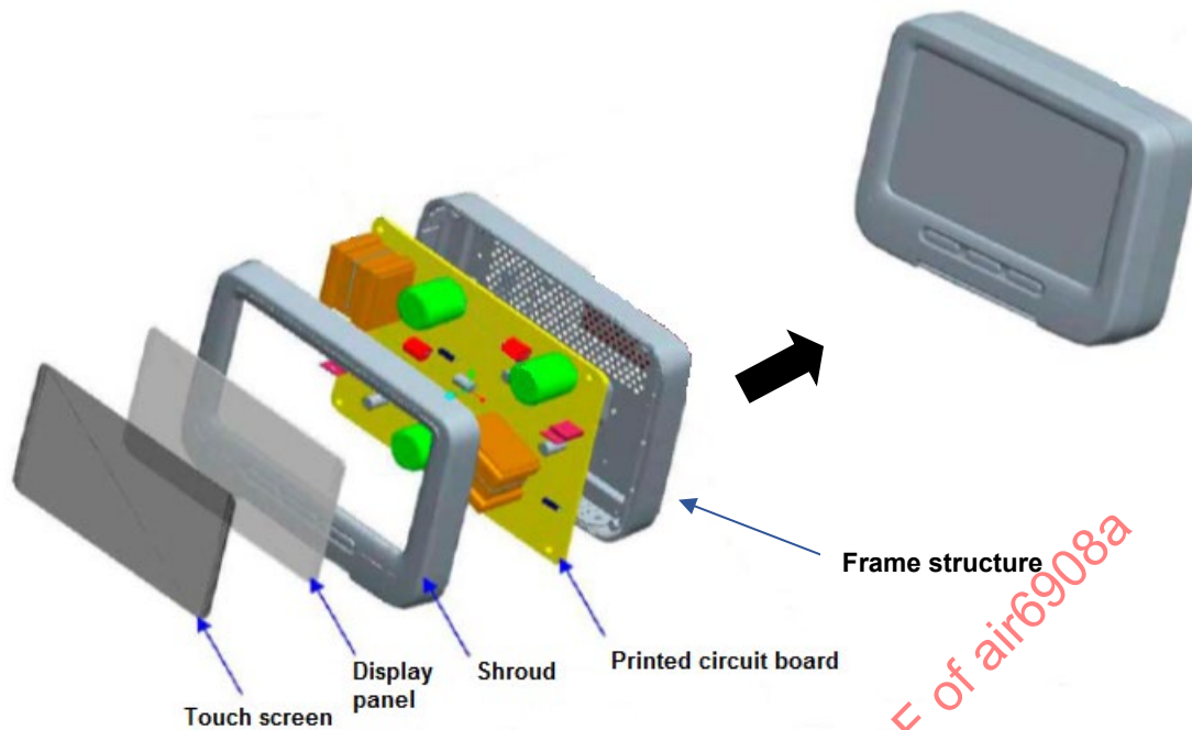
Figure 9 - Exploded view of IFE monitor (example)
