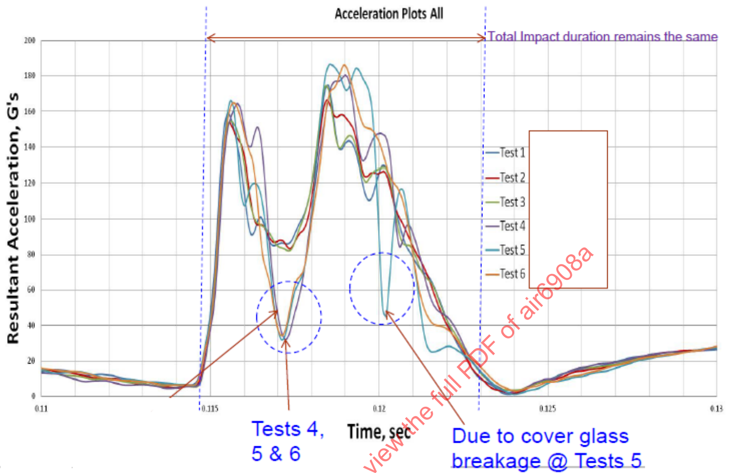
Figure E2 - Configuration #5 ATD head c.g. resultant acceleration
