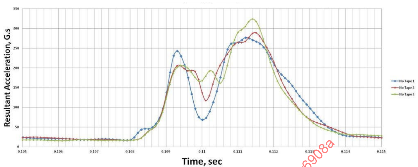
Figure I1 - Head acceleration over time, baseline monitor, impact location #1
