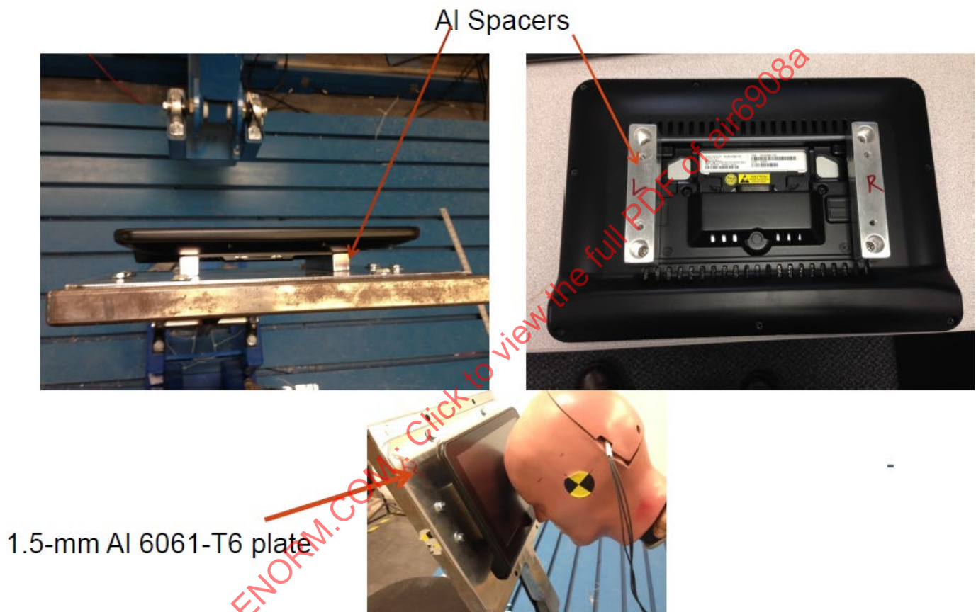
Figure E1 - Panasonic 11.1-inch monitor mounted to test fixture
