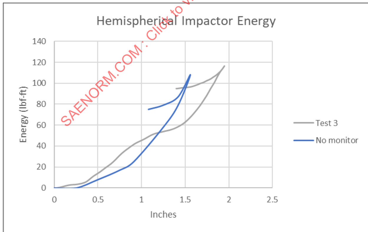
Figure 23 - Frangibility test impactor energy - with and without monitor
