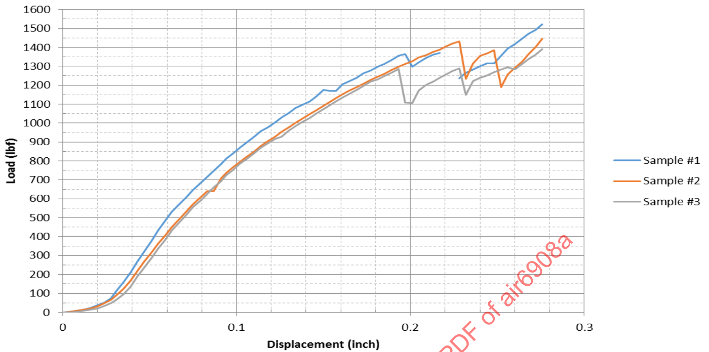
Figure F5 - Panasonic 9-inch mass equivalent monitor three-point bend test data
