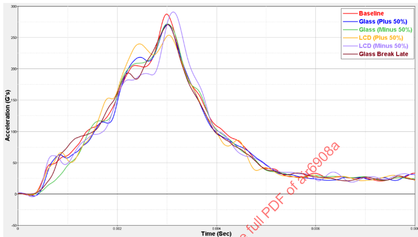
Figure G4 - Safran HCTD parametric study ATD head c.g. resultant acceleration with rigid bracket
