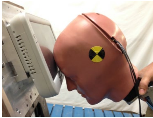
Figure 19 - Head component testing - bottom edge
