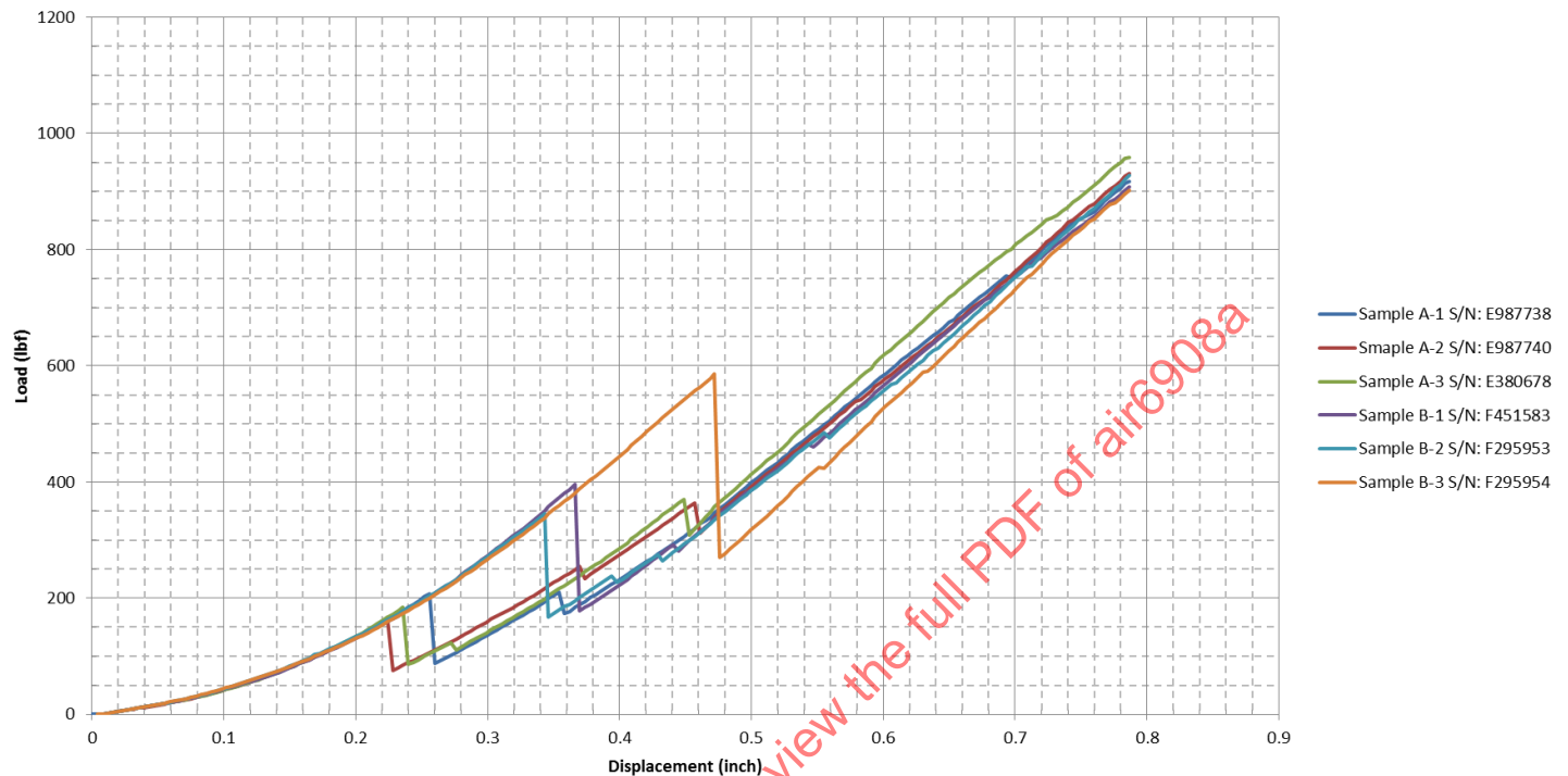
Figure F1 - Panasonic 10.6-inch monitor three-point bend test data
