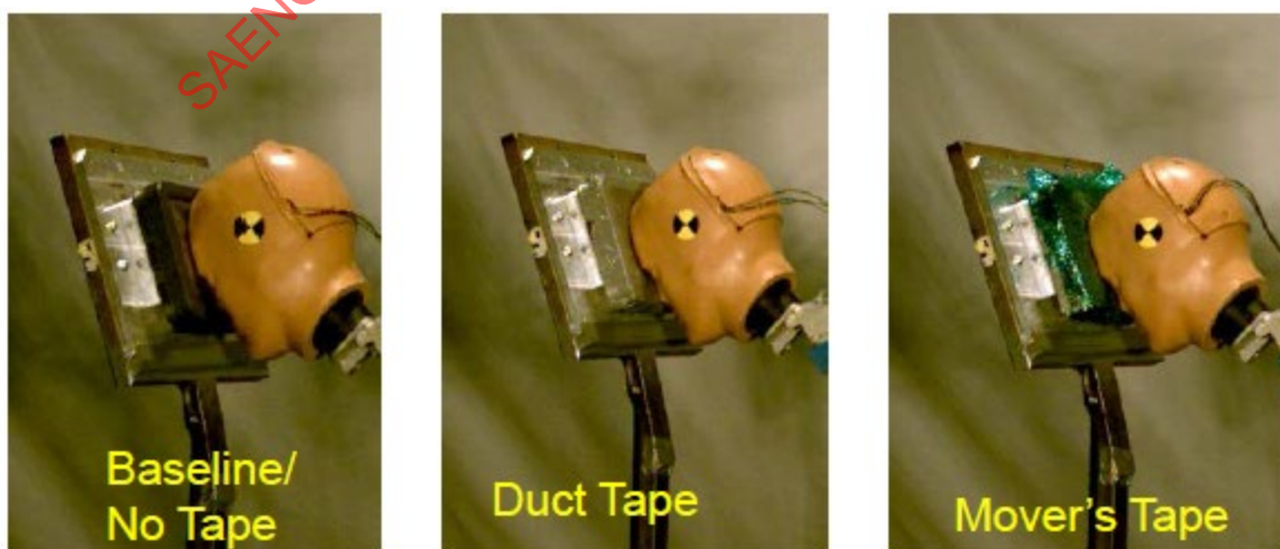
Figure 18 - Head component testing with added tape - center of view screen
