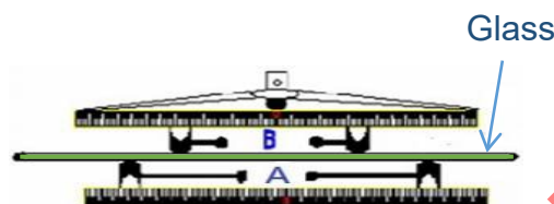
Figure 4 - Four-point bend test
