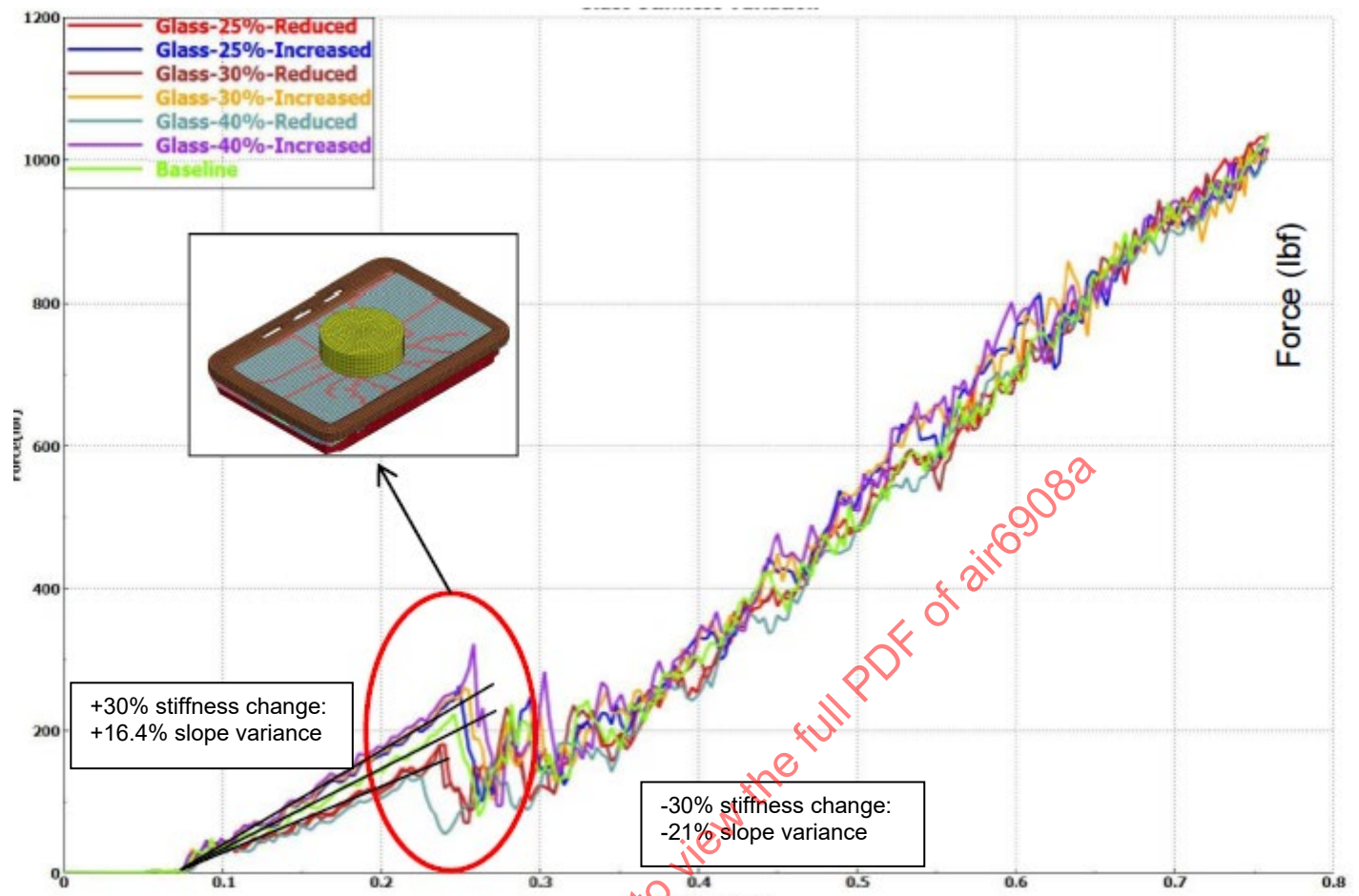
Figure 12 - Three-point bend test simulation - touch screen modulus of elasticity variance
