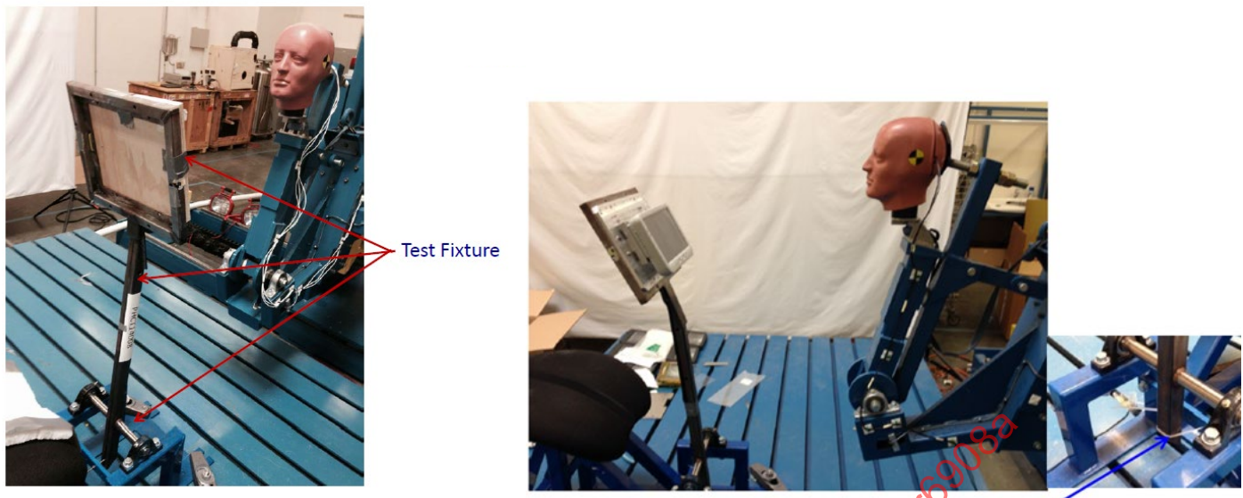
Figure 2 - Seat back test fixture
