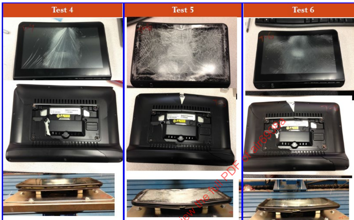
Figure E5 - Configuration #5 post-test photos of test 4, 5, and 6 monitors
