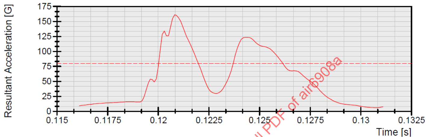
Figure E6 - Configuration #1 ATD head c.g. resultant acceleration
