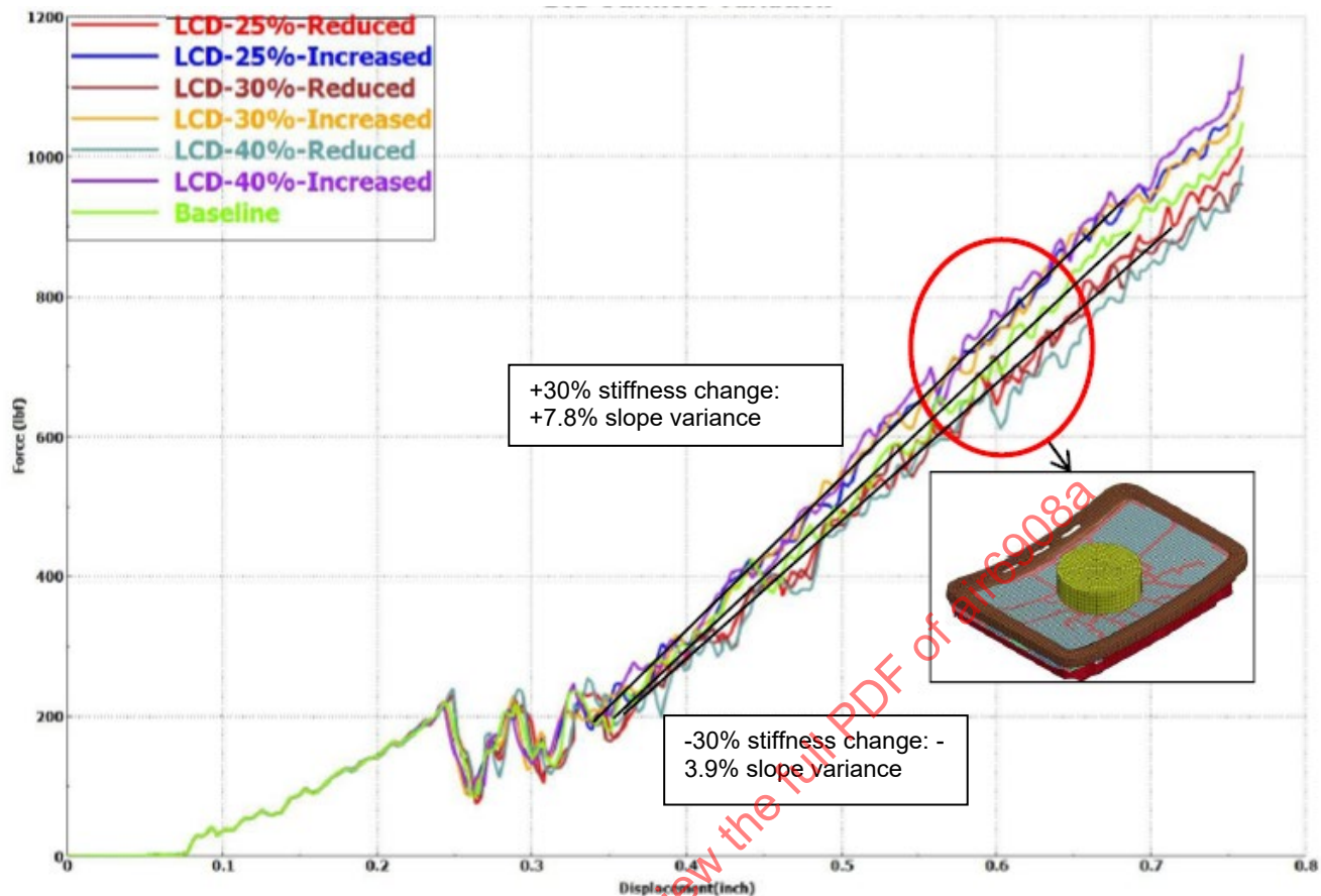
Figure 13 - Three-point bend test simulation - display panel modulus of elasticity variance
