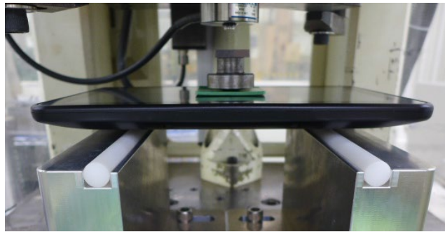
Figure 3 - Three-point bend test
