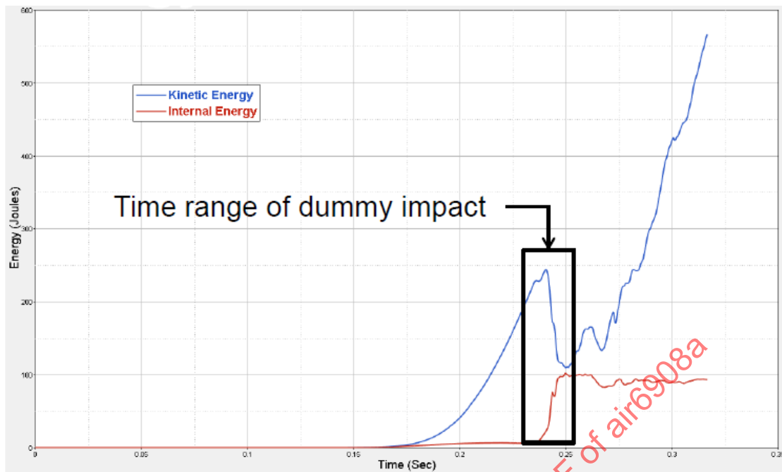
Figure H3 - Kinetic/internal strain energy attenuation over time - Safran
