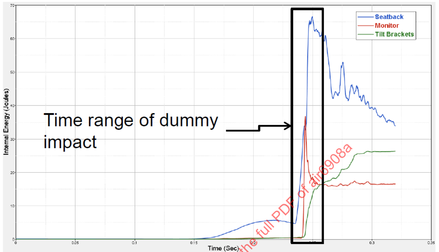
Figure H4 - Seat back internal strain energy distribution over time - Safran
