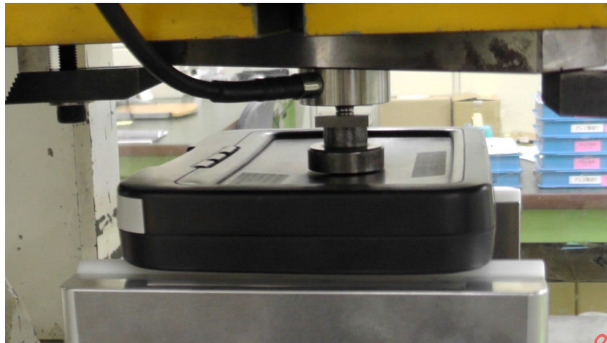
Figure F7 - Panasonic 9-inch mass equivalent monitor test - photo #2
