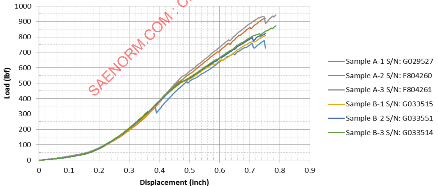
Figure F4 - Panasonic 11.1-inch monitor three-point bend test data
