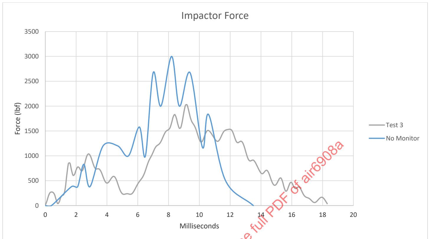
Figure 22 - Frangibility test impactor force - with and without monitor
