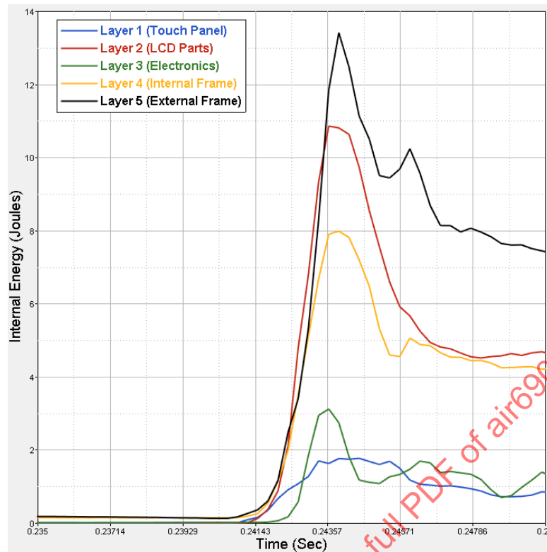
Figure H5 - Monitor internal strain energy distribution over time - Safran
