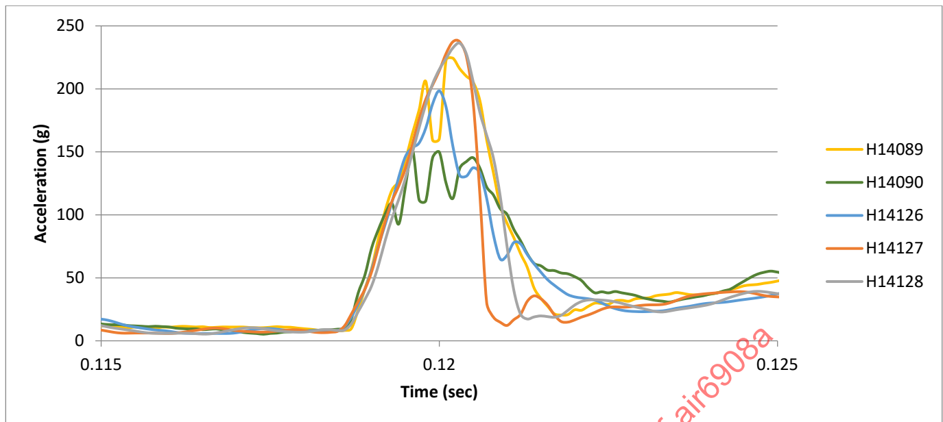
Figure C2 - Configuration #2 ATD head c.g. resultant acceleration
