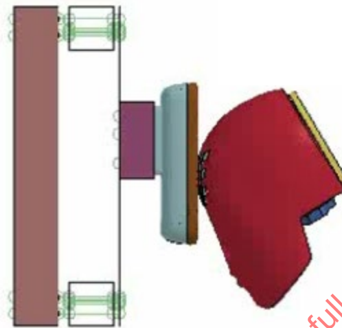
Figure J1 - Free motion headform simulation
