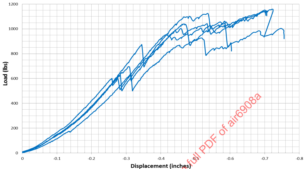
Figure F3 - Thales 8.9-inch monitor three-point bend test data
