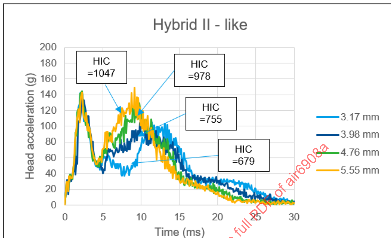
Figure J5 - Pendulum tester with Hybrid II type neck - simulation results
