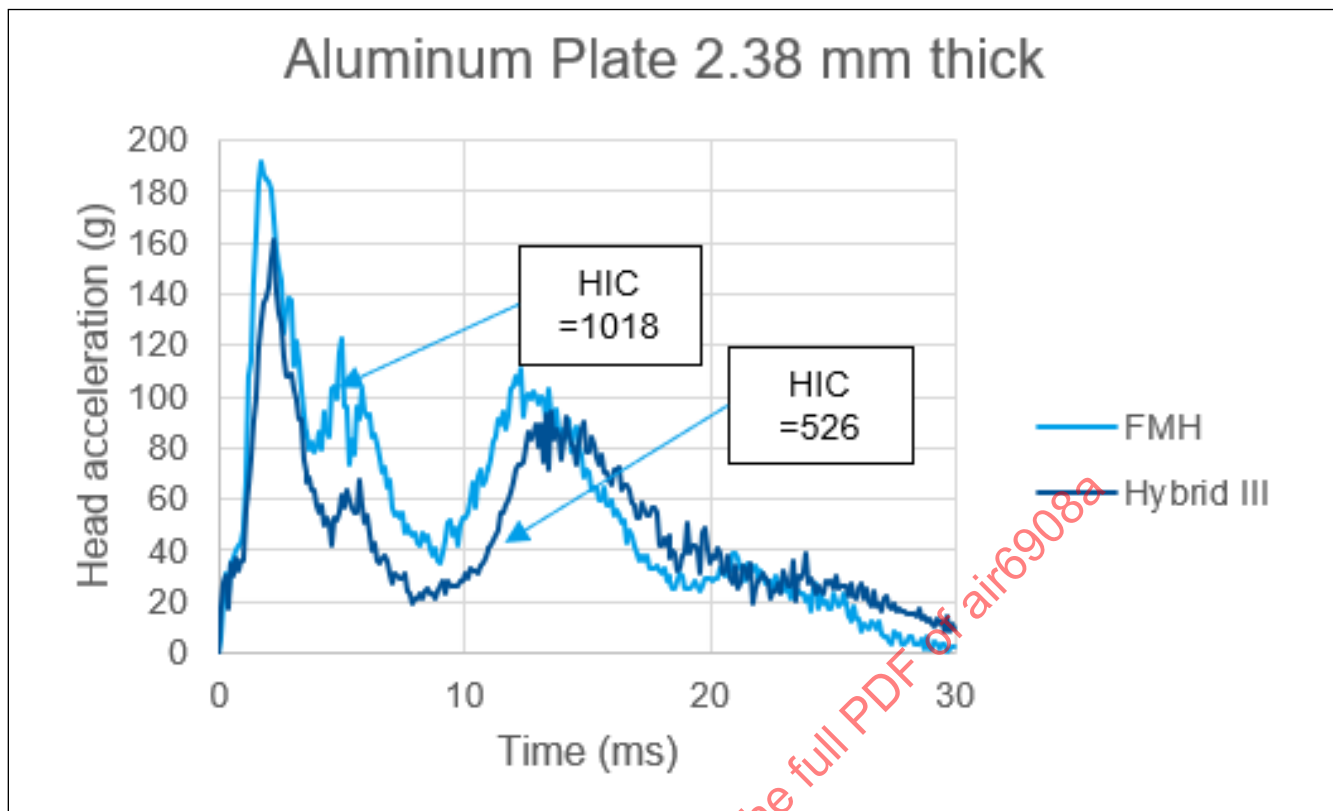
Figure J7 - Acceleration comparison between impactors - 2.38-mm aluminum thickness
