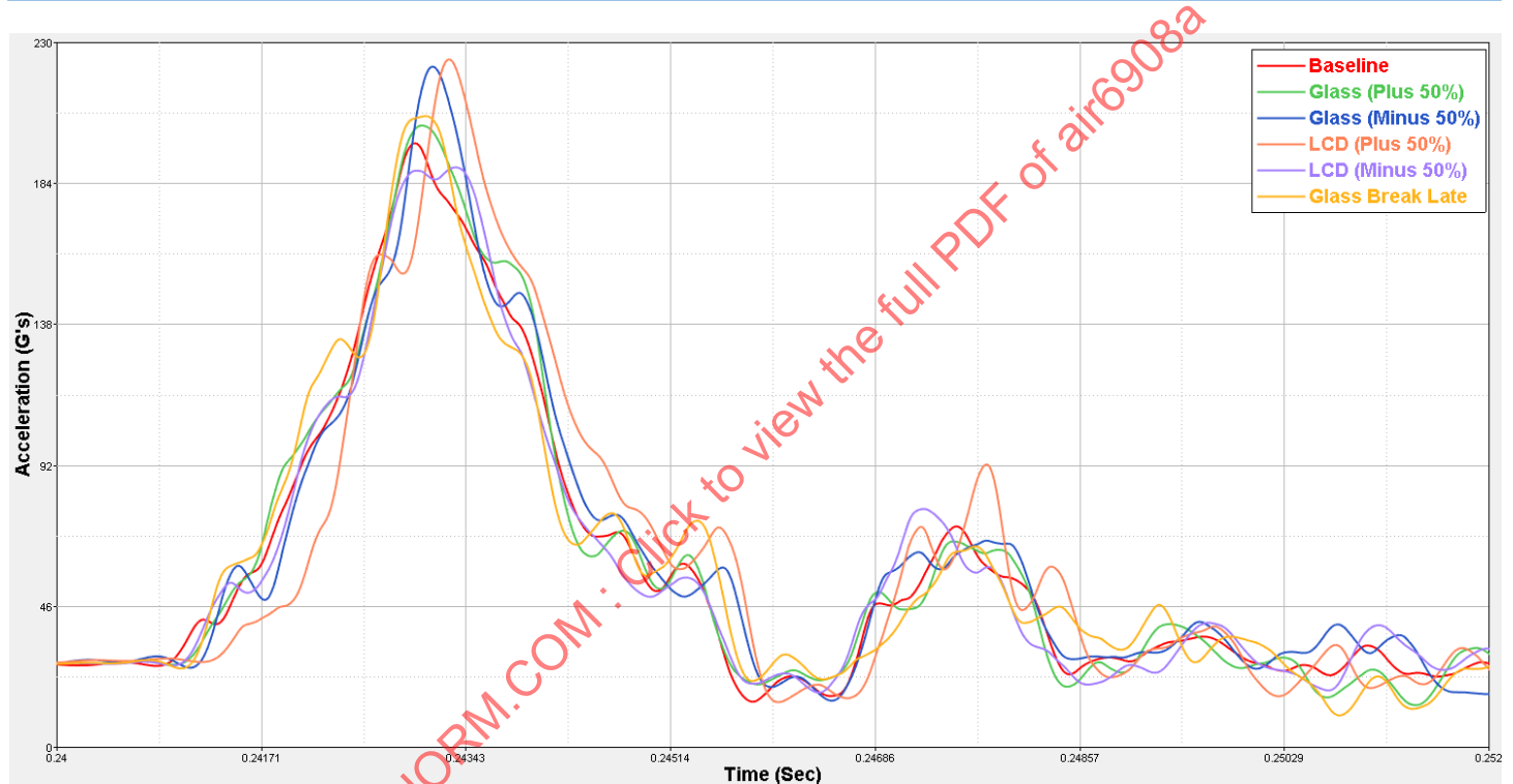
Figure G6 - Safran parametric study ATD head c.g. resultant acceleration for row-to-row dynamic tests
