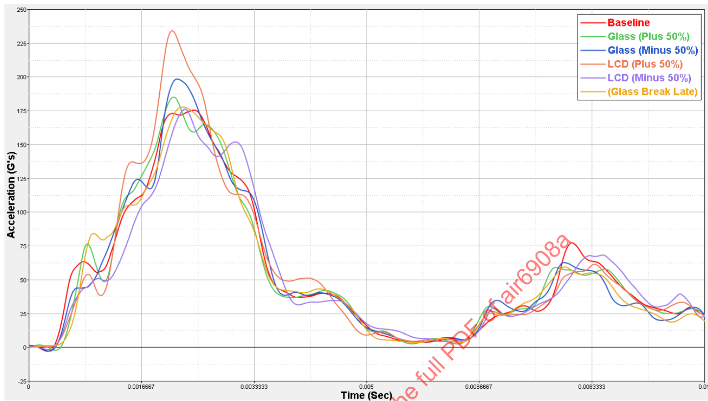
Figure G5 - Safran HCTD parametric study ATD head c.g. resultant acceleration with bracket tilt locked
