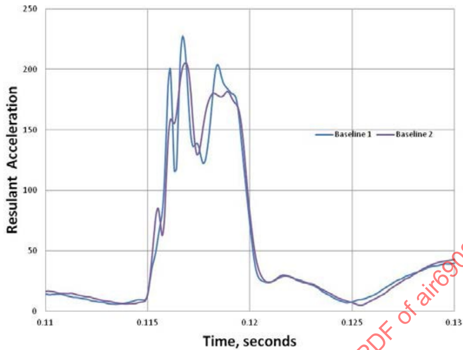
Figure I5 - Head acceleration over time, baseline monitor, impact location #2
