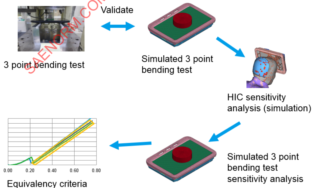
Figure 10 - HIC sensitivity analysis approach
