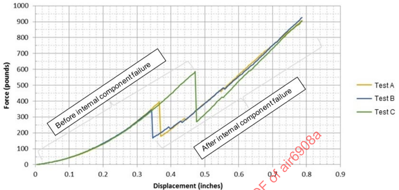
Figure 8 - Example IFE monitor force-displacement curve
