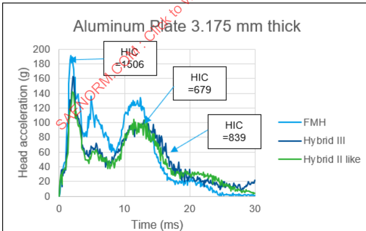
Figure J8 - Acceleration comparison between impactors - 3.175-mm aluminum thickness
