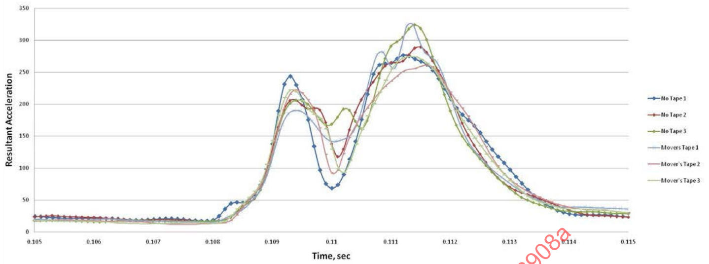
Figure I3 - Head acceleration over time, baseline versus mover's tape monitor configuration, impact location #1
