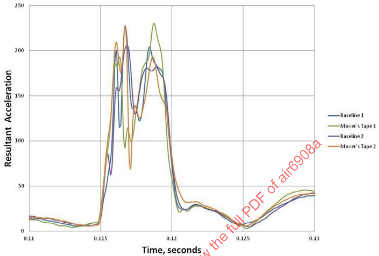
Figure 17 - Head acceleration over time, baseline versus mover's tape monitor configuration, impact location #2
