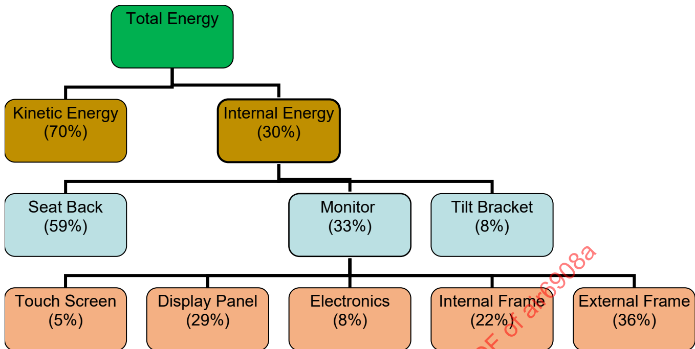
Figure 14 - Summary of seat back energy attenuation - Safran
