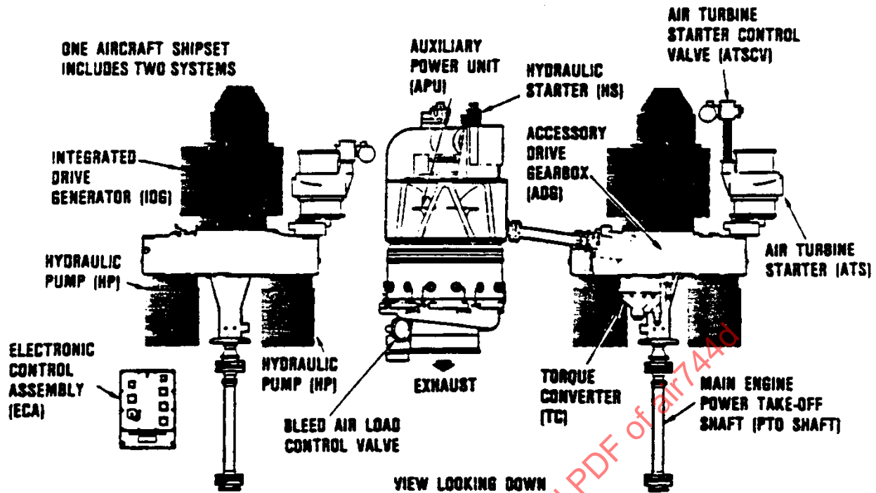
FIGURE 15 - SECONDARY POWER SYSTEM FOR U.S. AIR FORCE B-1B
