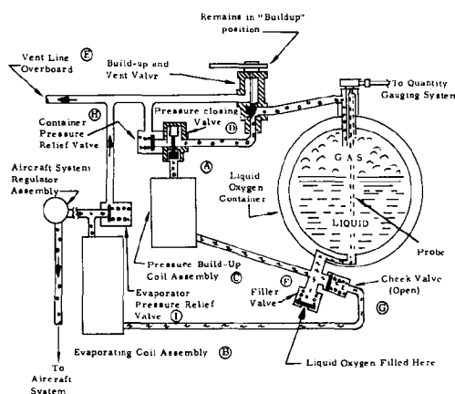
SYSTEM SUPPLY PROCEDURE FIGURE 2
