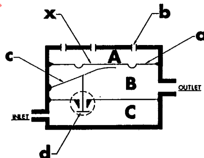
FIGURE I - TYPICAL DEMAND REGULATOR
