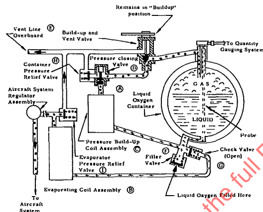
SYSTEM SUPPLY PROCEDURE FIGURE 2
