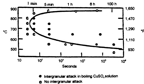
FIGURE 1 - Effect of Time and Temperature on Sensitization of 18.2% Cr, 11.0% Ni, 0.05% C, 0.05% N Stainless Steel
