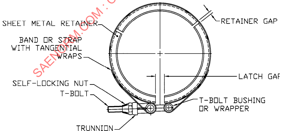
FIGURE 5 - V-BAND COUPLING
