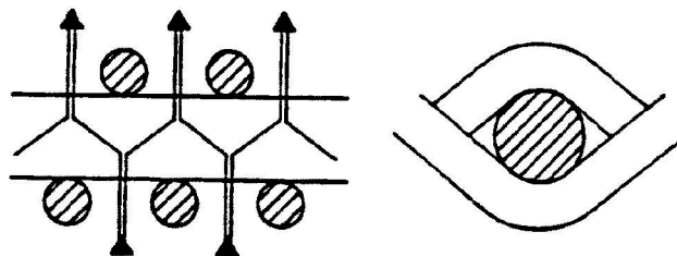
FIGURE 8 - Plain Dutch Single Weave Tortuosity Factor - 1.9
