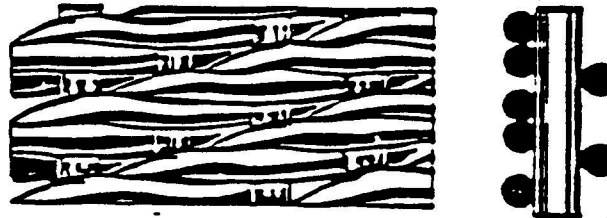
FIGURE 5 - Twilled Dutch Single Weave
