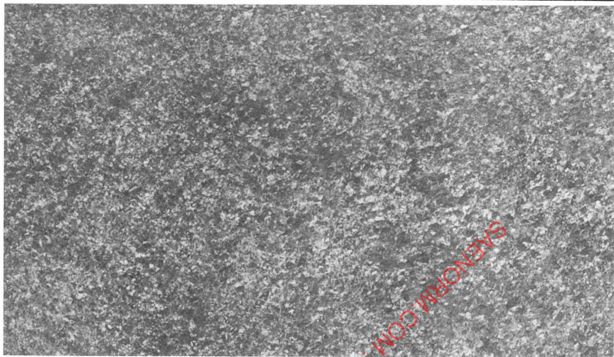
Acceptable, Fine Macro-grain, Uniform Macrostructure FIGURE 14
