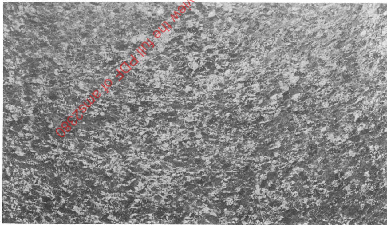
Acceptable, Medium Macro-grain, Uniform Macrostructure FIGURE 15
