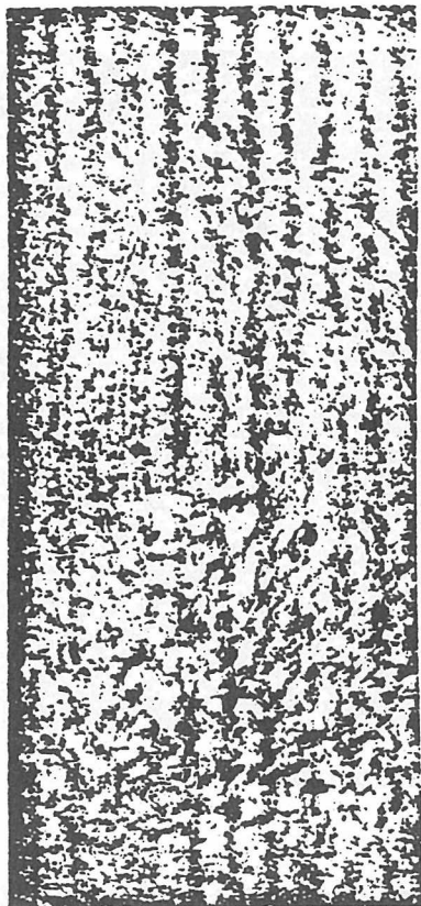
Unacceptable Porosity FIGURE 12
