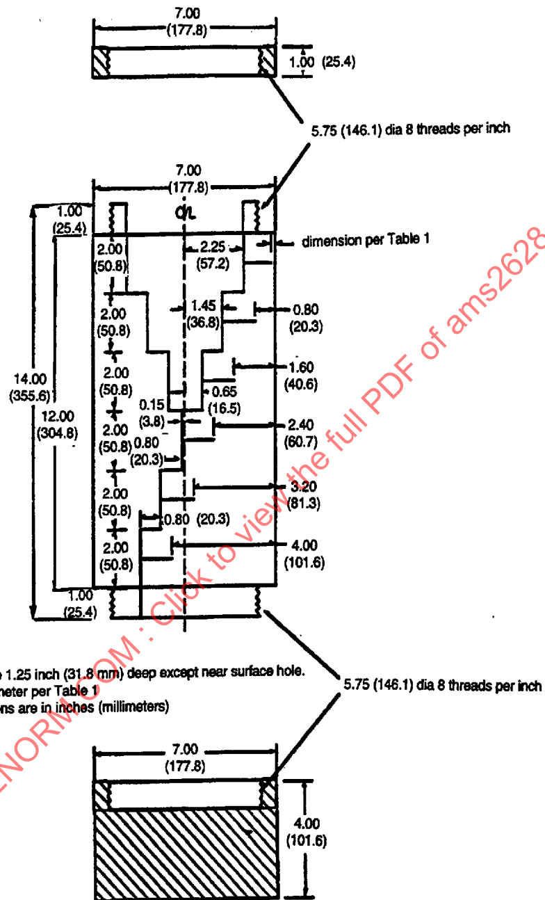
FIGURE C3 - Titanium Calibration Standard, 7.0 Inches (178 mm) Diameter
