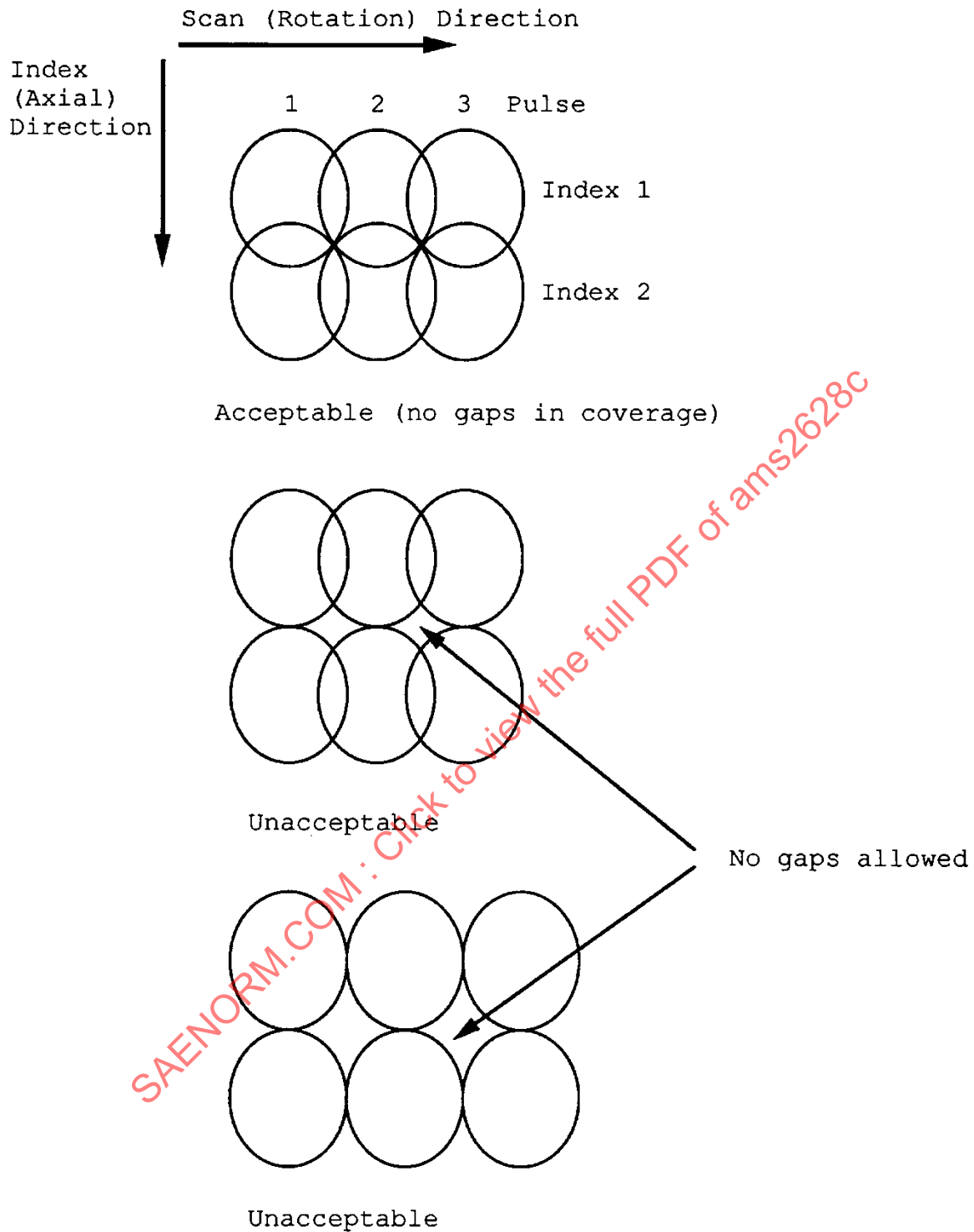
Figure 1 - Acceptable beam overlap conditions in accordance with 3.5.3.1
