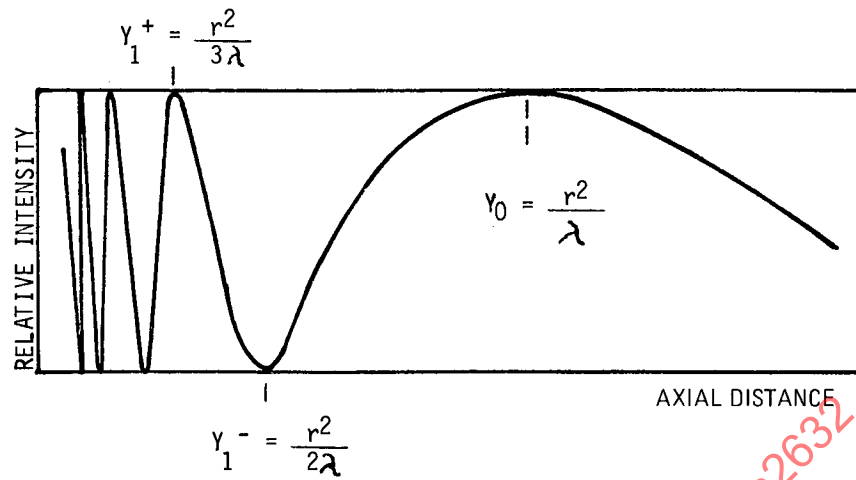
SEARCH UNIT AXIAL DISTANCE AMPLITUDE CURVE (Profile for Flat Piston Radiator)
