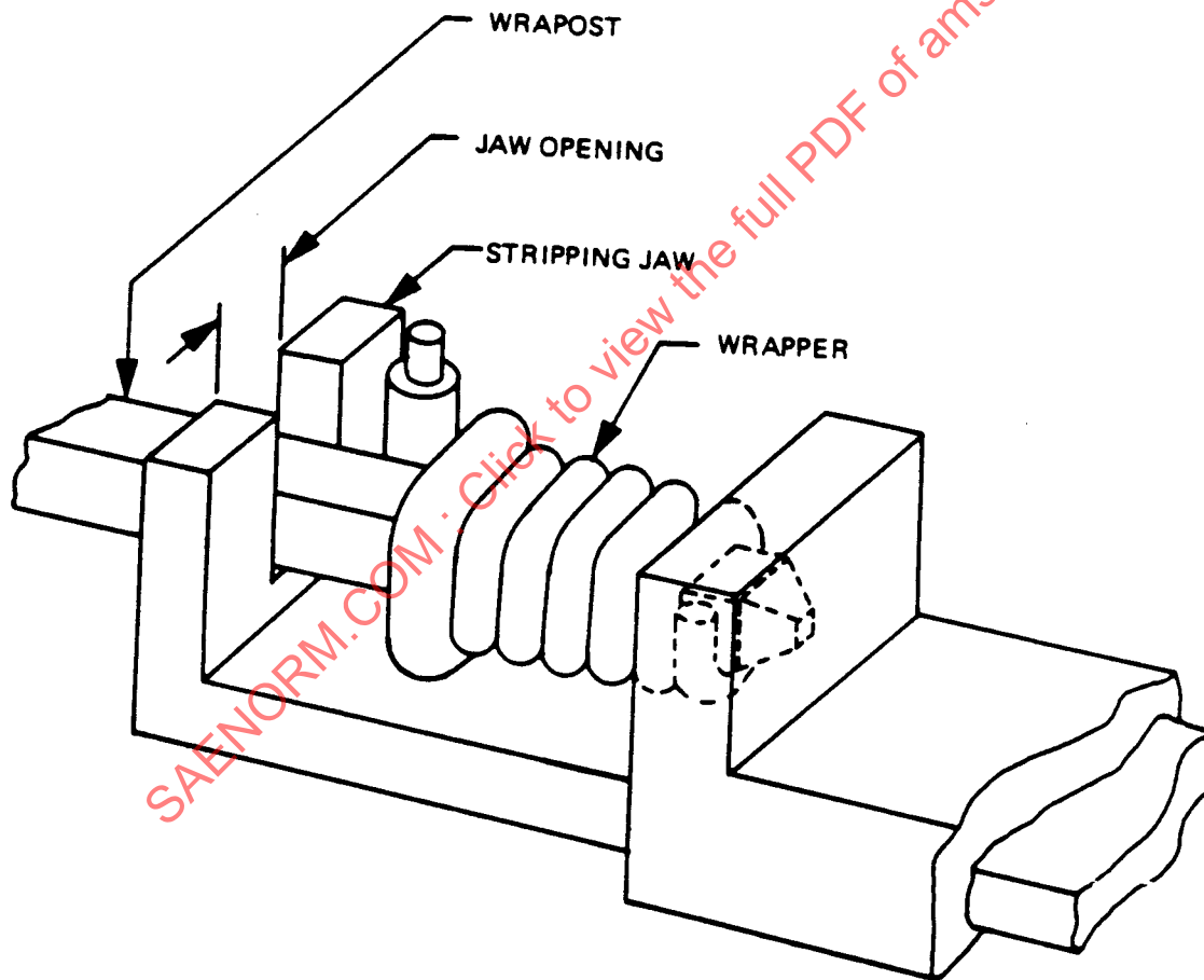
FIGURE 3 - Stripping Test Fixture
