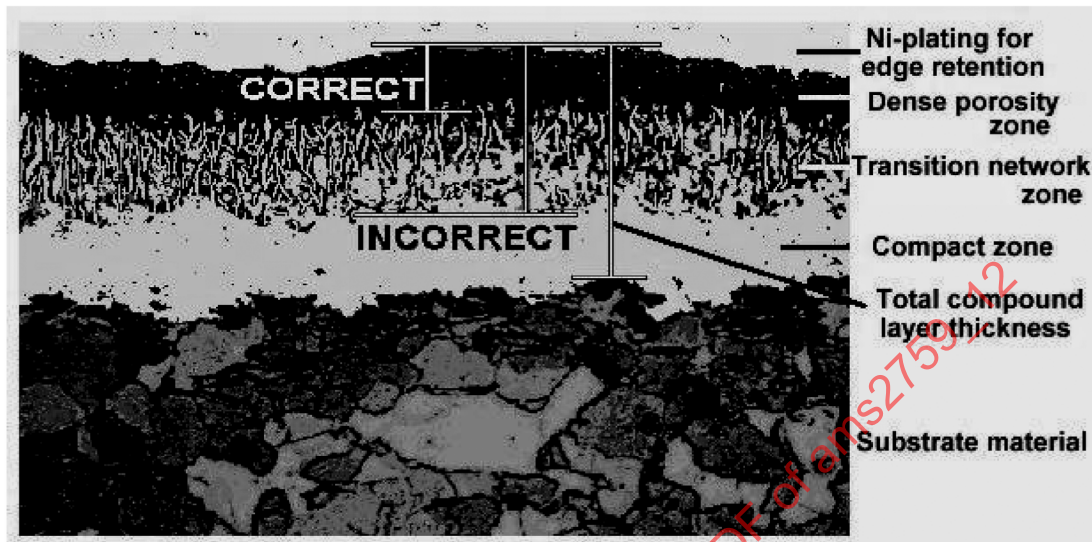
FIGURE 1 - EVALUATION OF EXTENT OF POROSITY IN COMPOUND LAYER ON NON-ALLOYED STEEL
