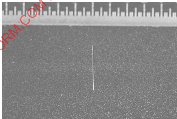
Figure 2 - Example indication from a fatigue crack specimen. The indication is crisp and clearly discernible. Background fluorescence is low. Scale: major divisions: 2.5 mm (0.1 inch).
