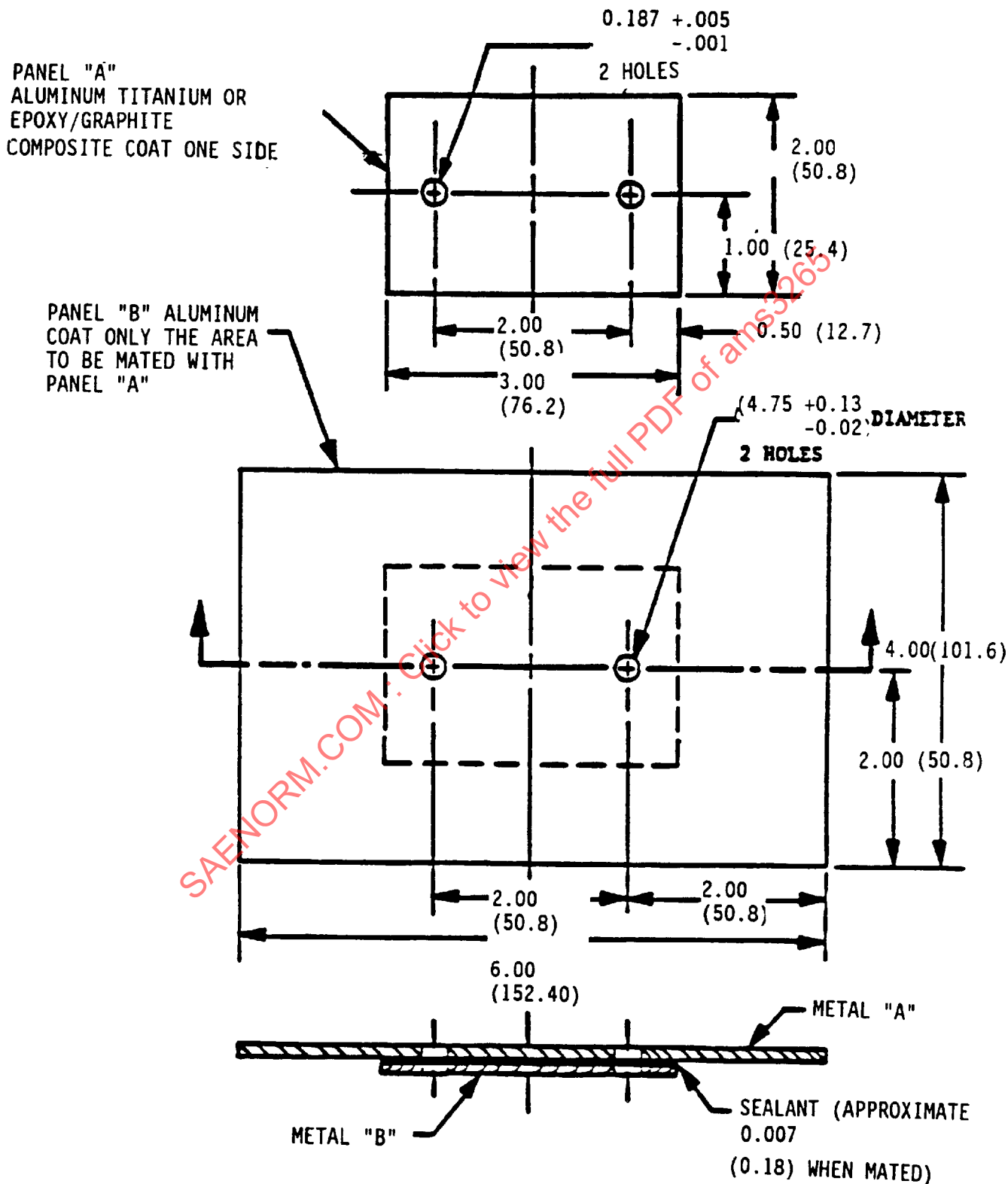
FIGURE 6 - Mixed Couple Assembly
