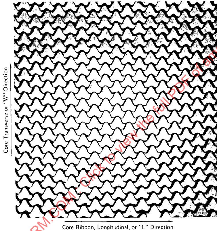
FIGURE 1 - FLEXIBLE CORE CONFIGURATION
