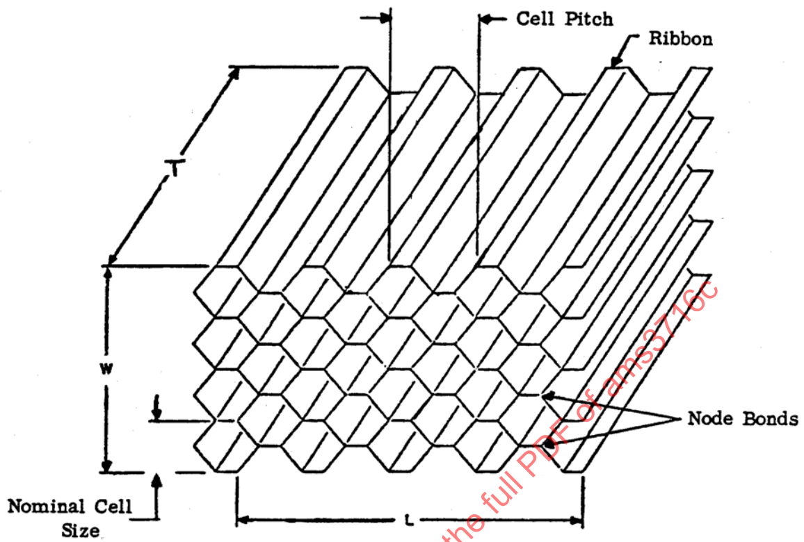
FIGURE 1 - Honeycomb Core
