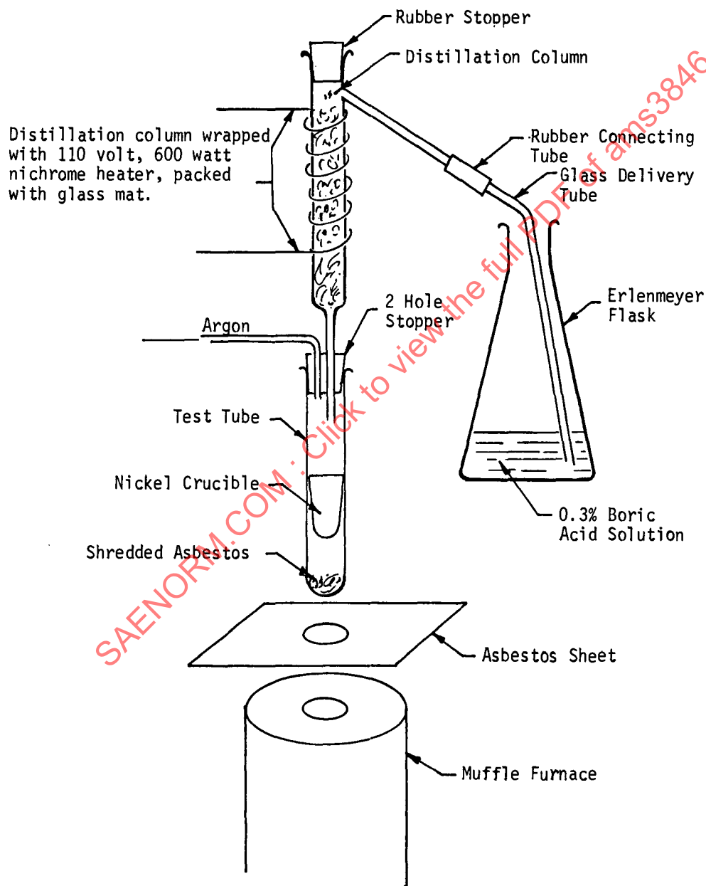
APPARATUS FOR ANALYSIS OF QUARTZ FINISH
