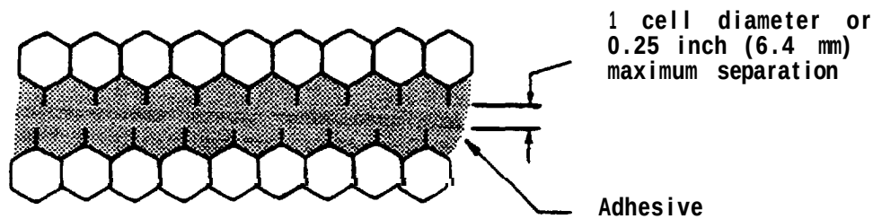
Figure 3 - Core Splice (Type 2 Structure)
