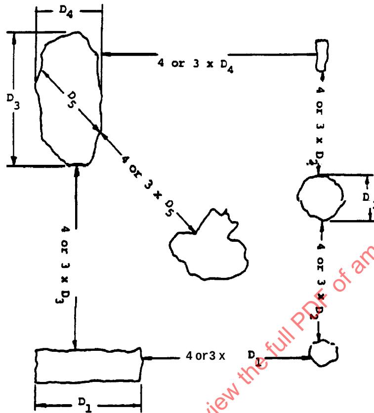
FIGURE 2 - Measuring Disbond Spacing
