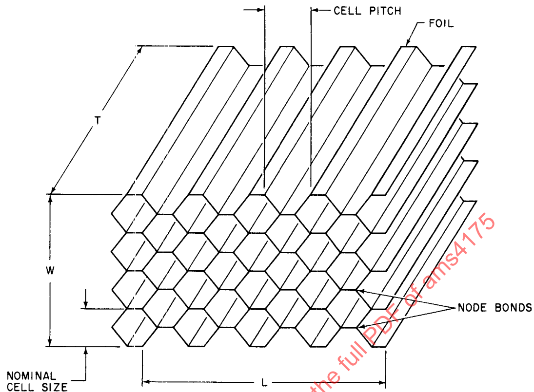
Honeycomb Core
