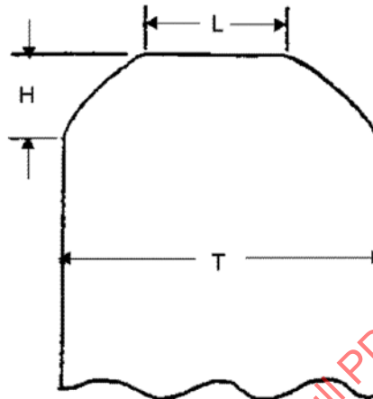
FIGURE 1 - WIRE ROUNDED EDGES
