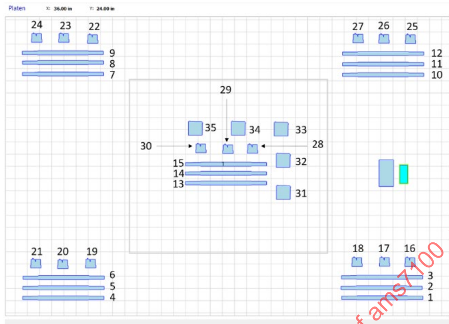
Figure 2 - Process control document (PCD) build arrangement of 15 ASTM D638 tensile coupons in the XZ orientation (parts 1 to 15 in image), 15 ASTM D638 tensile coupons in the ZX orientation (parts 16 to 30), and five density cubes (parts 31 to 35) spread across five build locations
