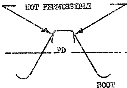
FIGURE 5 ROLLED THREAD
