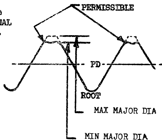
FIGURE 9 ROLLED THREAD
