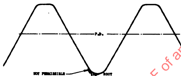
FIGURE 3 ROLLED THREAD
