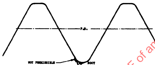
Figure 4 Rolled Thread
