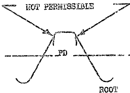
Figure 6 Rolled Thread
