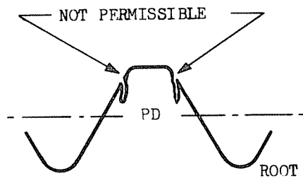
ROLLED THREAD FIGURE 6
