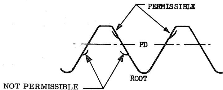
ROLLED THREAD FIGURE 7
