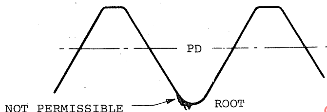
ROLLED THREAD FIGURE 4
