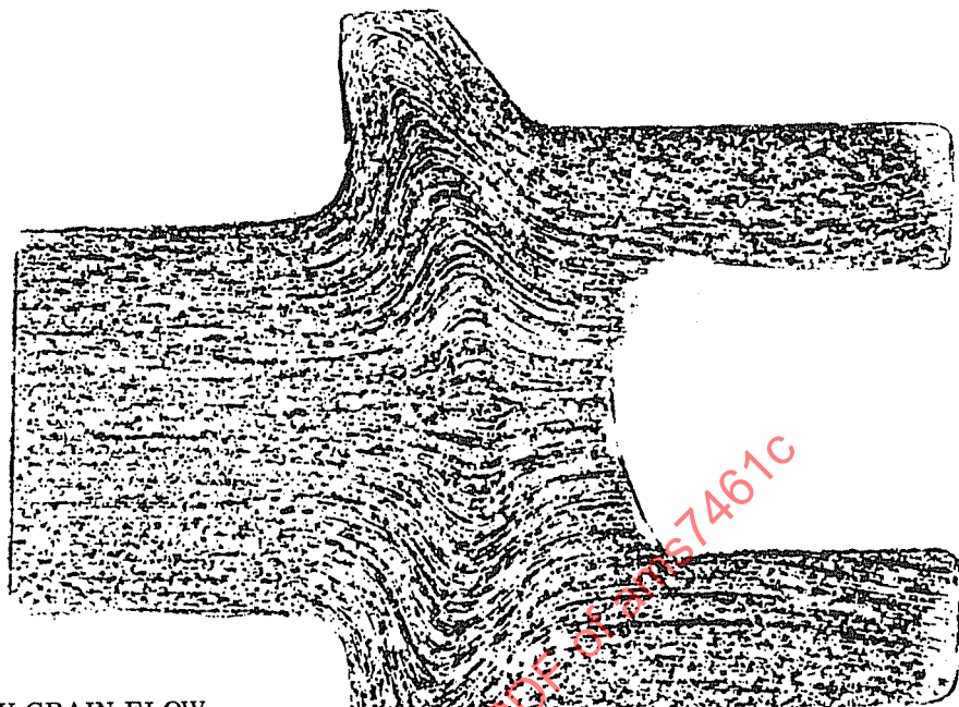
SATISFACTORY GRAIN FLOW FIGURE 1A
