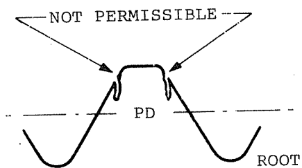
ROLLED THREAD FIGURE 6
