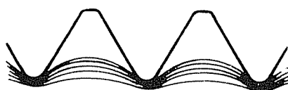
FLOW LINES, ROLLED THREAD FIGURE 3
