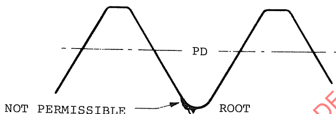
ROLLED THREAD FIGURE 4
