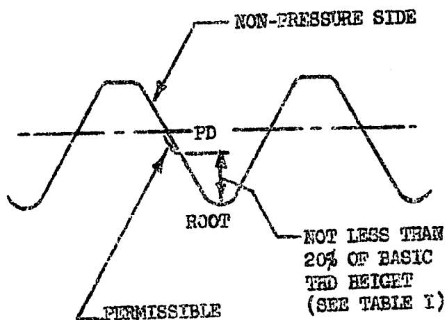
Ø FIGURE 6 ROLLED THREAD
