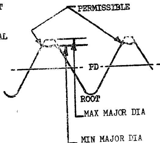
FIGURE 9 ROLLED THREAD
