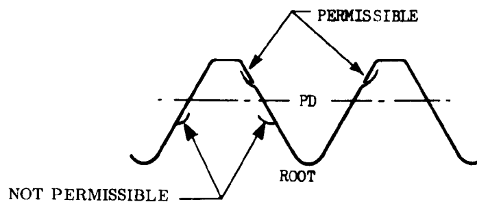
ROLLED THREAD FIGURE 7
