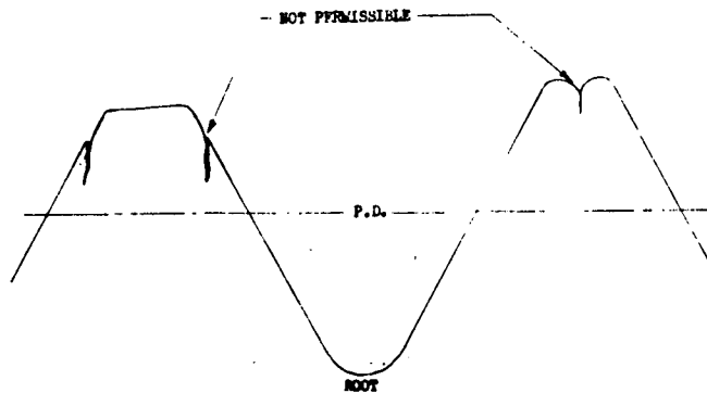
FIGURE 5 ROLLED THREAD
