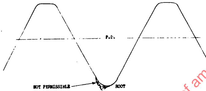
FIGURE 3 ROLLED THREAD
