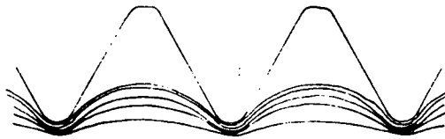
FIGURE 2 ROLLED THREAD
