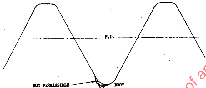
FIGURE 3 ROLLED THREAD
