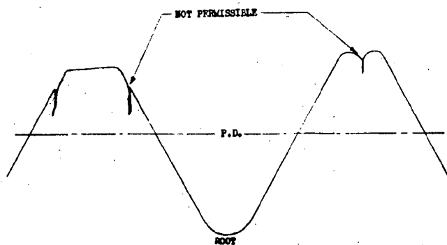
FIGURE 5 ROLLED THREAD
