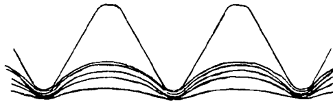
FIGURE 2 TYPICAL ROLLED THREAD
