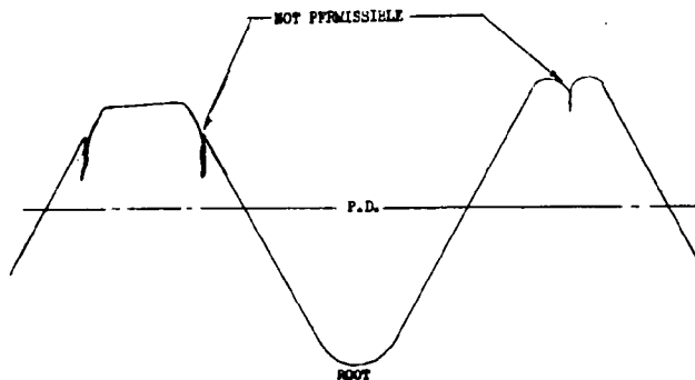
FIGURE 5 ROLLED THREAD
