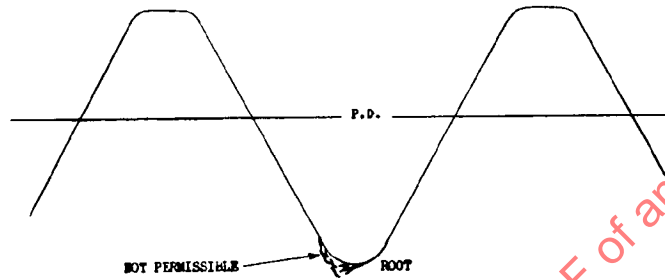
FIGURE 3 ROLLED THREAD
