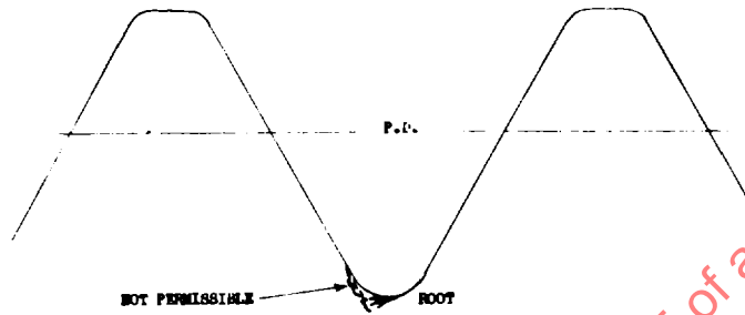
FIGURE 3 ROLL-ON THREAD
