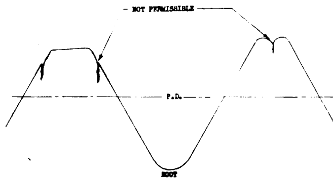
FIGURE 5 ROLL-ON THREAD
