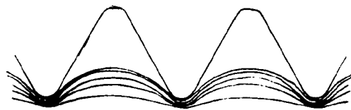
FIGURE 2 NON PERMISSIBLE ROLLED THREAD
