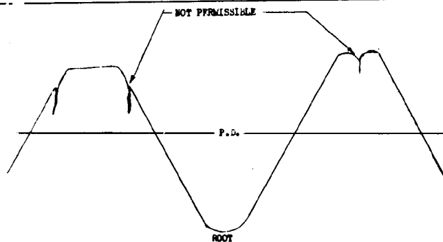
FIGURE 5 ROLLED THREAD
