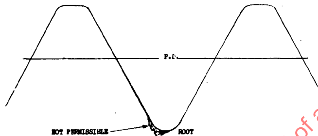
FIGURE 3 ROLLED THREAD
