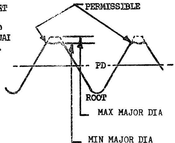
FIGURE 8 ROLLED THREAD
