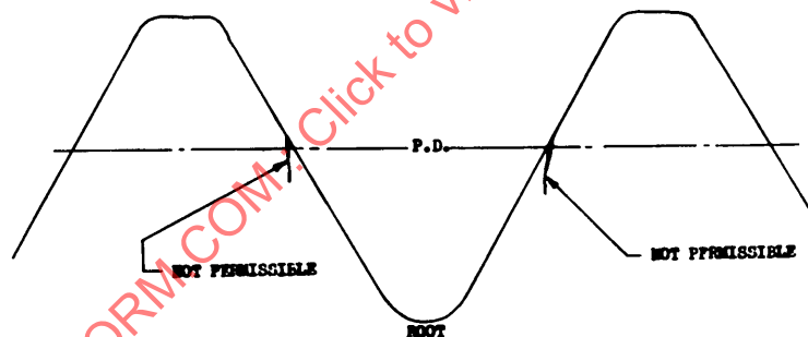
FIGURE 3 ROLLED THREAD
