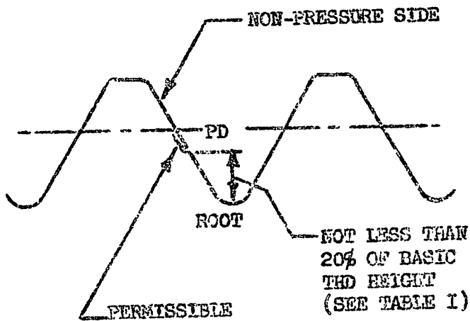
Ø FIGURE 5 ROLLED THREAD
