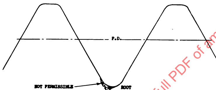
FIGURE 2 ROLLED THREAD
