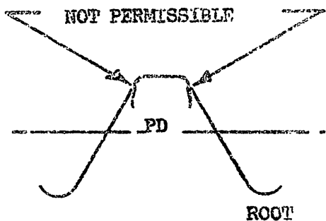
Ø FIGURE 4 ROLLED THREAD
