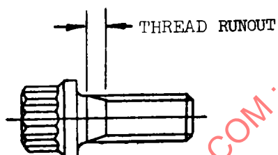
FULL SHANK THREADED TO HEAD
