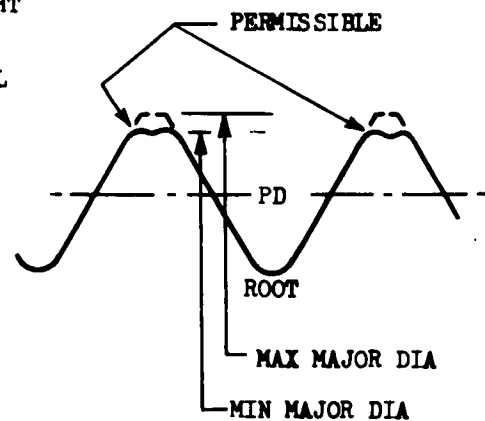
ROLLED THREAD FIGURE 9
