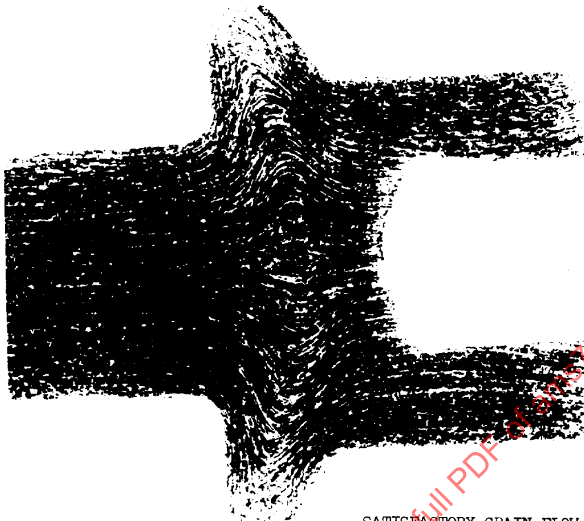
SATISFACTORY GRAIN FLOW FIGURE 1A
