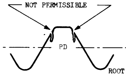
ROLLED THREAD
