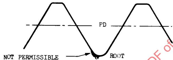
ROLLED THREAD
