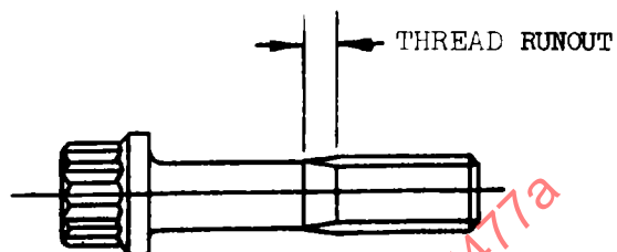
RELIEVED SHANK
