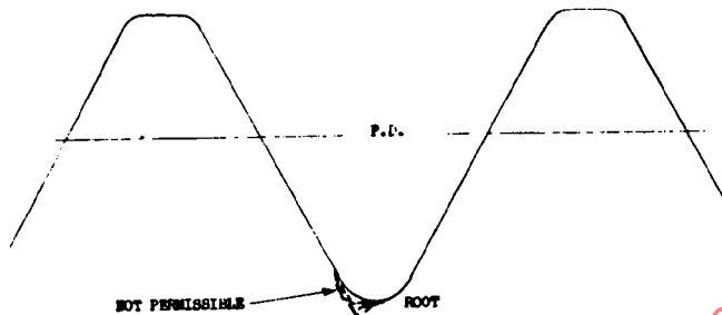
FIGURE 3 ROLLED THREAD
