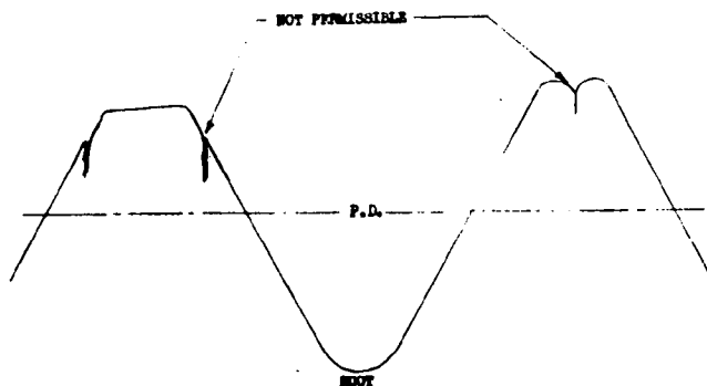
FIGURE 5 ROLLED THREAD
