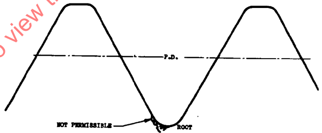
FIGURE 3 ROLLED THREAD
