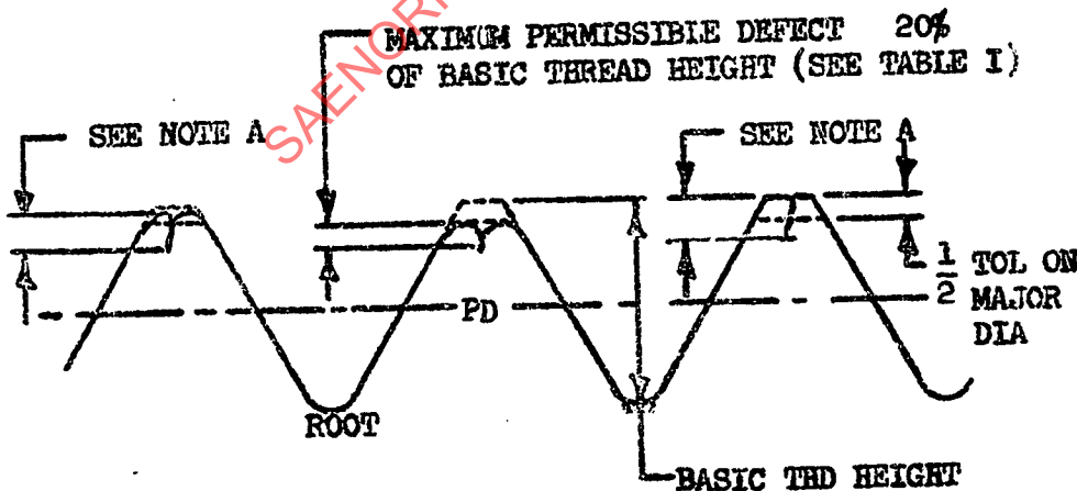
FIGURE 7 ROLLED THREAD
