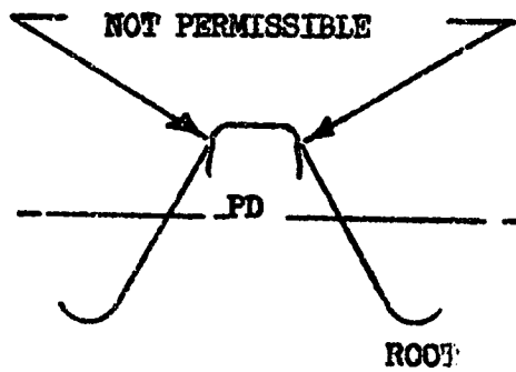
FIGURE 5 ROLLED THREAD
