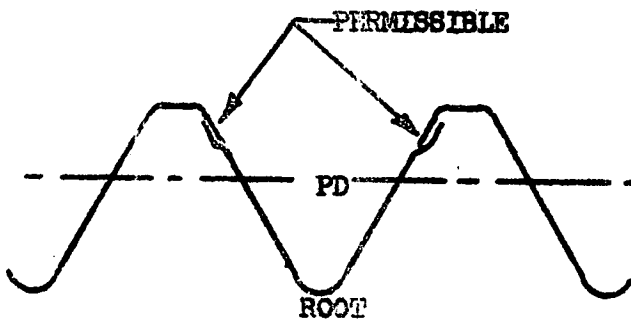
FIGURE 5 ROLLED THREAD
