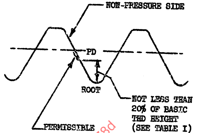
FIGURE 6 ROLLED THREAD
