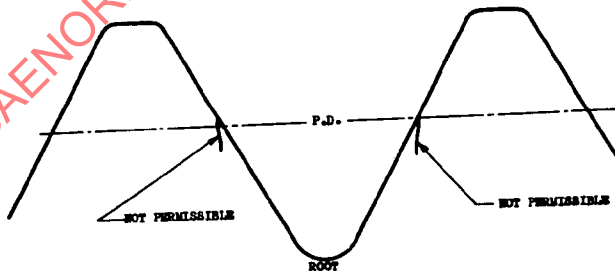
FIGURE 4 ROLLED THREAD
