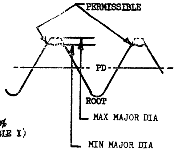
FIGURE 9 ROLLED THREAD
