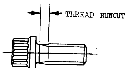
RELIEVED SHANK THREADED TO HEAD
