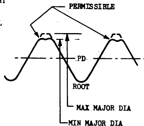
ROLLED THREAD FIGURE 8
