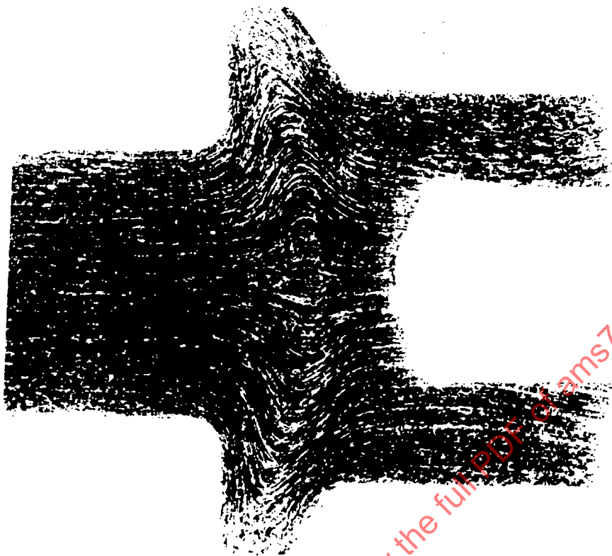
SATISFACTORY GRAIN FLOW FIGURE 1A
