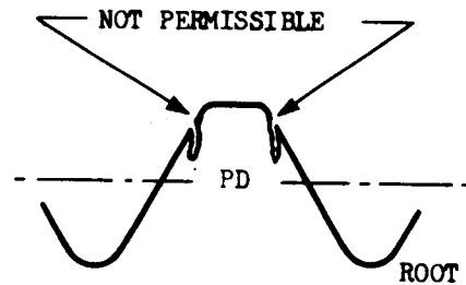
ROLLED THREAD FIGURE 5
