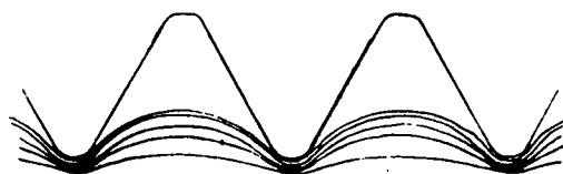
FIGURE 2 ROLLED THREAD
