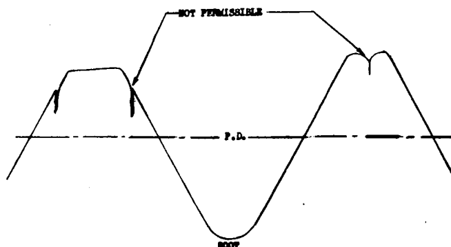
FIGURE 5 ROLLED THREAD
