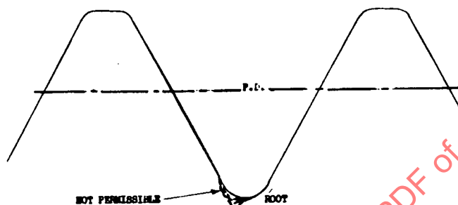
FIGURE 3 ROLLED THREAD
