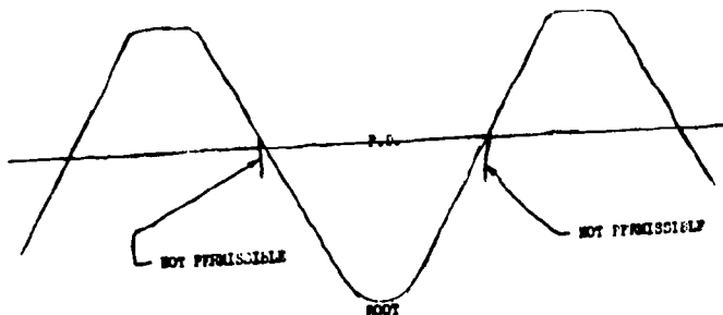
FIGURE 4 NOT PERMISSIBLE ROLLED THREAD
