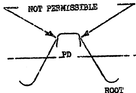
FIGURE 5 ROLLED THREAD
