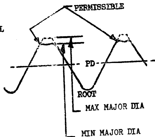
FIGURE 9 ROLLED THREAD
