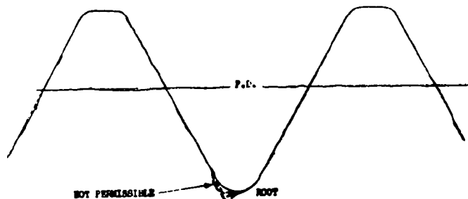
FIGURE 3 NOT PERMISSIBLE ROLLED THREAD
