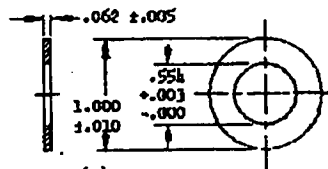
(c) WASHER
