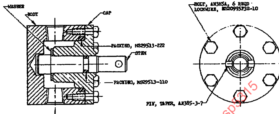
(a) PACKING TEST JIG
