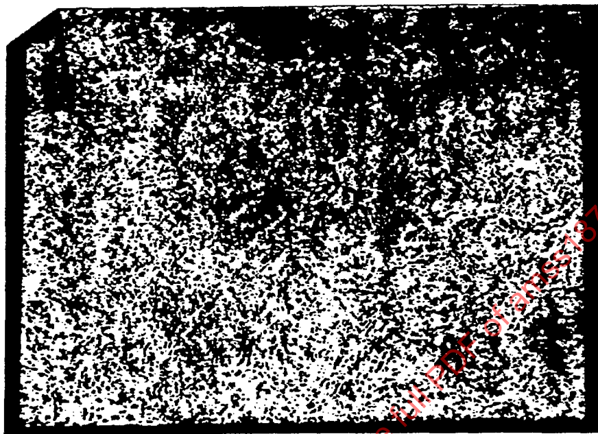
FIGURE 5 - Acceptable microstructure containing maximum amount of banded retained austenite permitted in any field of examination
